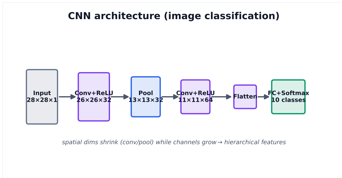
Figure 4. Convolution + pooling progressively reduce spatial size while increasing channel depth, building features from edges → textures → objects, then a dense head classifies.
