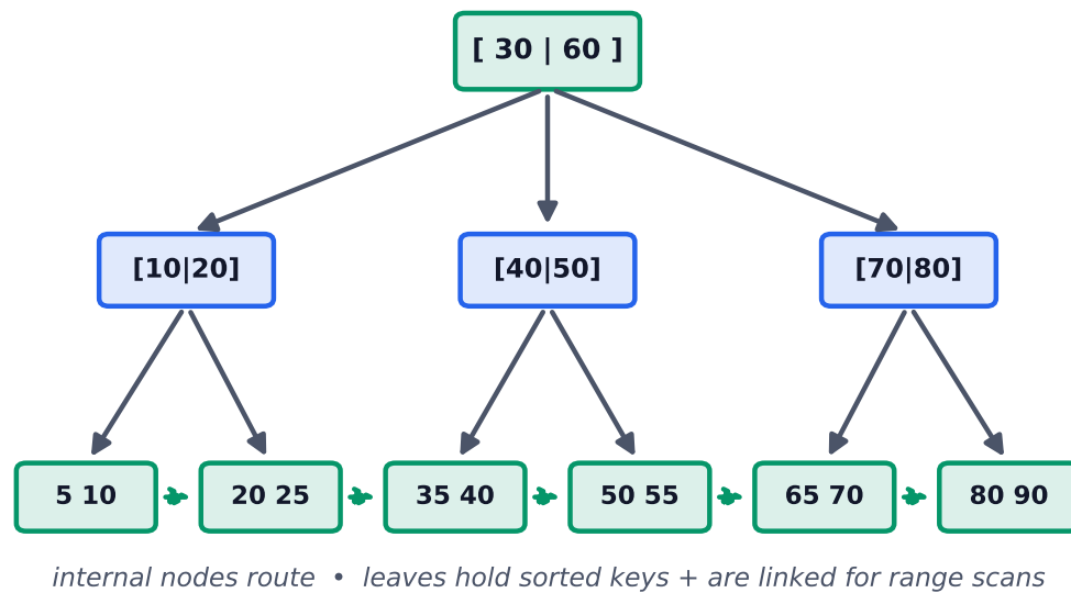
Figure 1. B+ trees keep data sorted with a high branching factor, so lookups touch only O(\log n) nodes (few disk pages). Linked leaves make range queries cheap.
