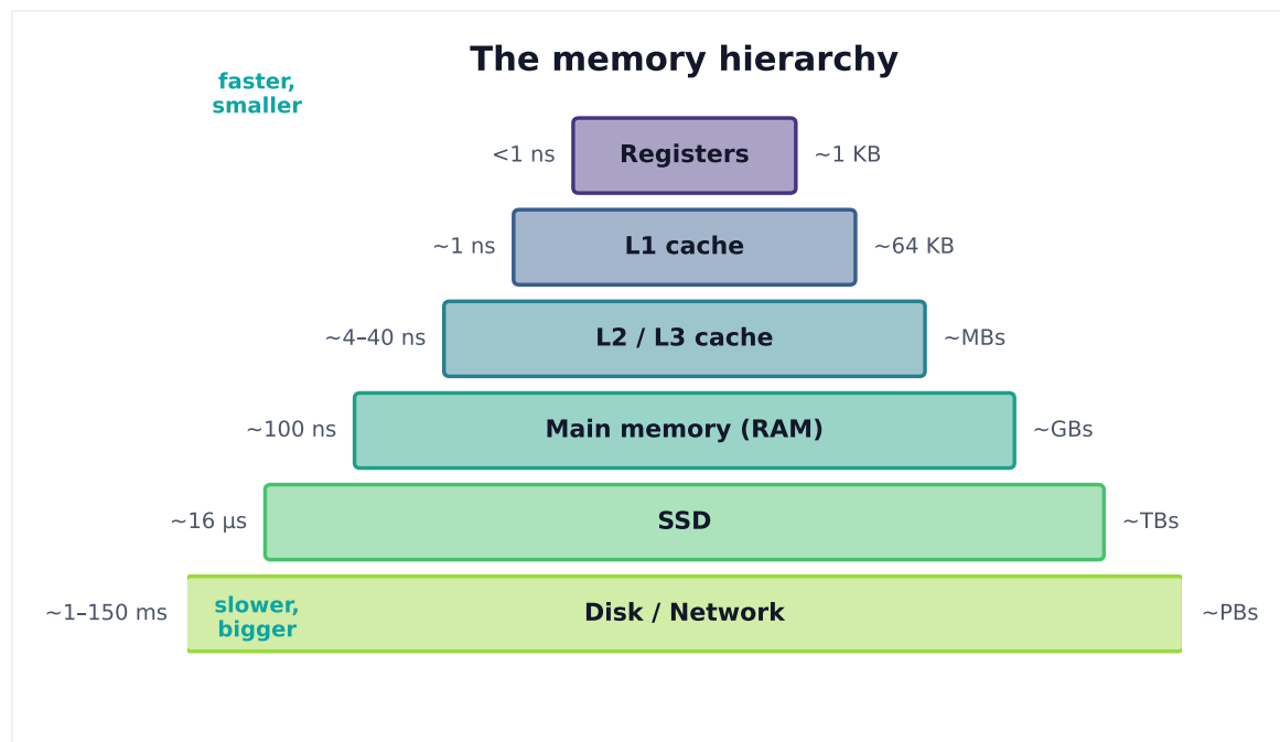
Figure 3. Each level trades capacity for speed by orders of magnitude. Performance comes from keeping the working set in the fastest tier that fits — the basis of caching.
