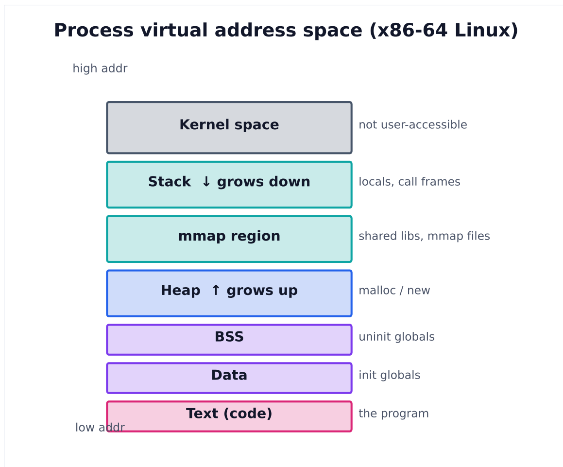
Figure 2. A process sees a flat virtual address space: code and globals at the bottom, the heap growing up and the stack growing down toward each other, kernel mapped on top.
