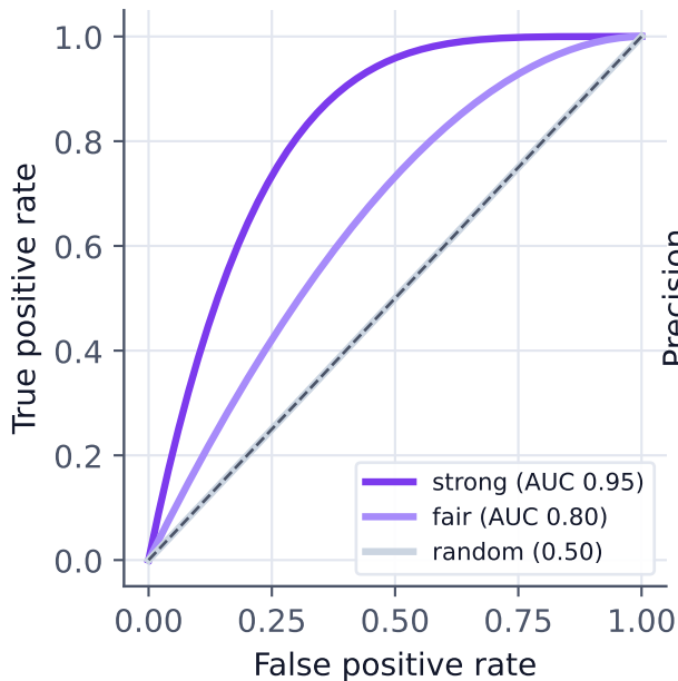
ROC curve
