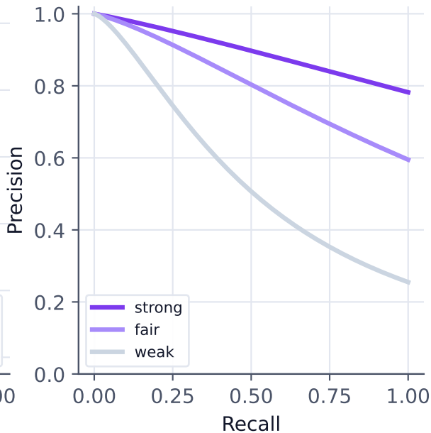
Precision-Recall curve
