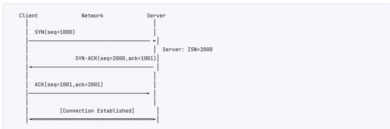
Figure 2. TCP opens with SYN / SYN-ACK / ACK to agree on sequence numbers, then tears down with a four-way FIN/ACK exchange. This reliability is what UDP trades away for speed.
