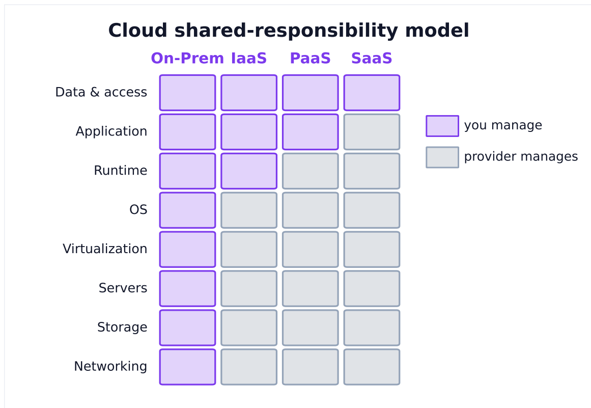
Figure 1. Moving from IaaS to SaaS hands more of the stack to the provider. Knowing the boundary tells you what you must still secure, patch and scale yourself.
