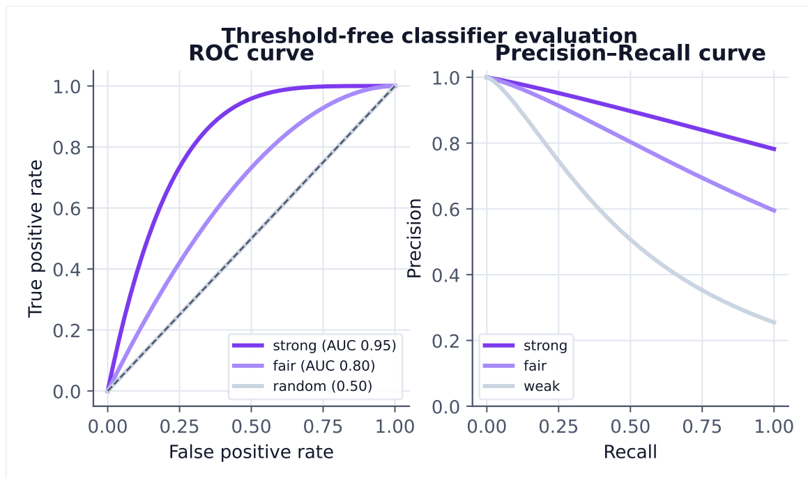
Figure 1. ROC summarizes ranking quality across thresholds; PR is more informative under heavy class imbalance, where a high AUC can still hide poor precision.
