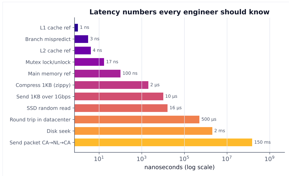
Figure 2. Orders of magnitude separate cache, memory, SSD, disk and network. Designing for performance means counting which tier each operation touches.
