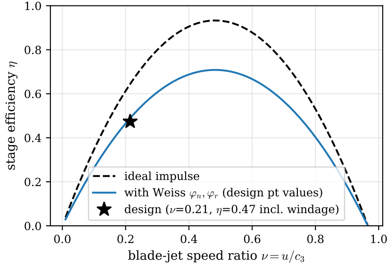
Figure 6: Impulse stage efficiency against blade to jet speed ratio. The dashed line is the ideal impulse stage of eq. (36), the solid line includes the Weiss loss coefficients evaluated at the design point, and the star marks the design point of this turbine, far below the optimum speed ratio.
