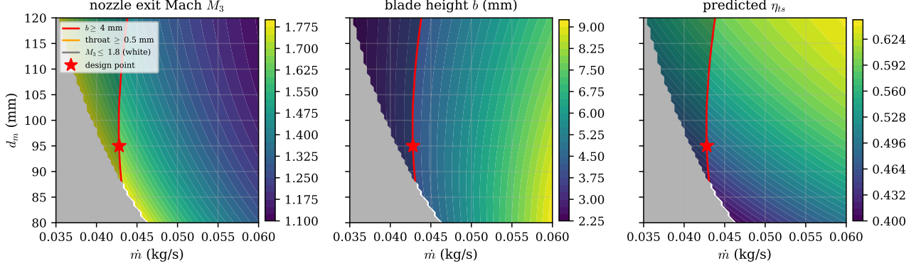
Figure 17: The turbine design space over mean diameter and mass flow, evaluated with the full sizing and loss model at the design speed. The panels show nozzle exit Mach number, blade height and predicted total to static efficiency. Overlaid lines are the design constraints (blade height \geq 4 mm, nozzle throat \geq 0.5 mm, M_3 \leq 1.8 ), the shaded region is infeasible, and the marker is the selected design point.
