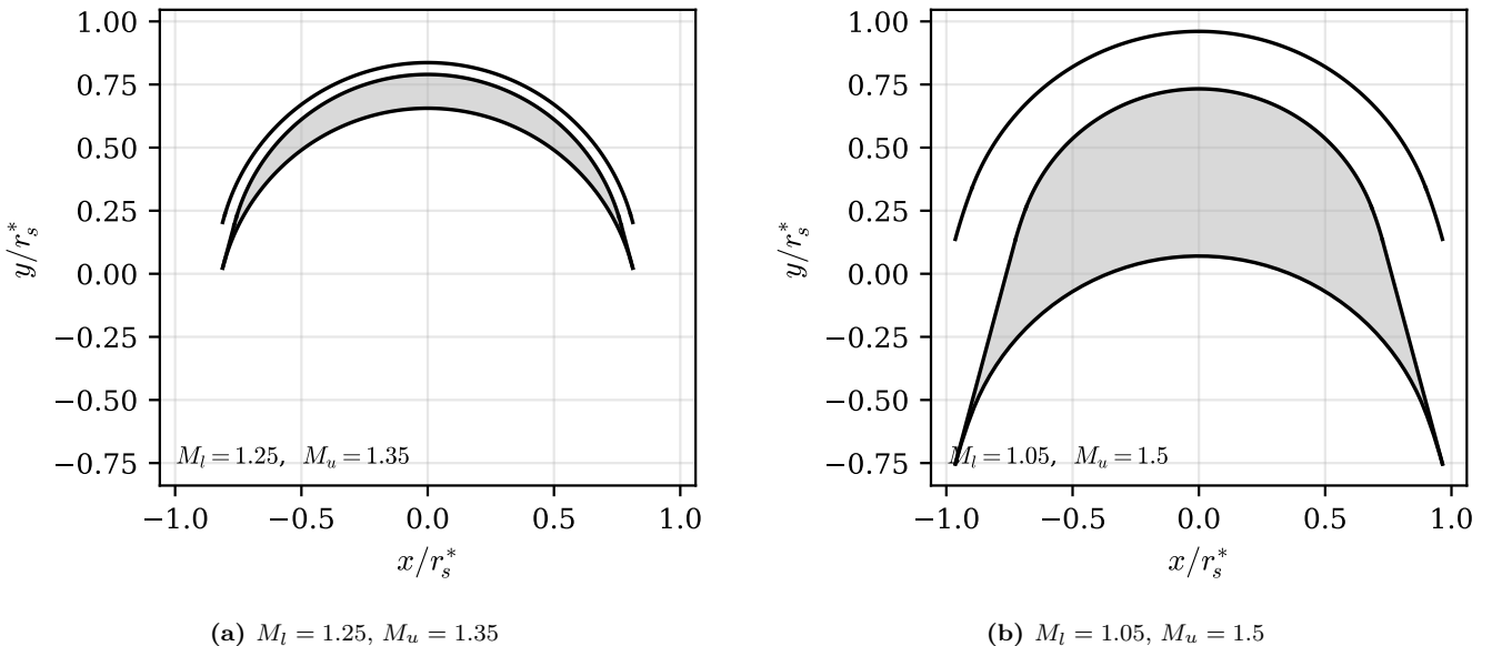
Figure 11: The effect of surface Mach number spread on the blade passage, for the same inlet conditions and shared axis scales. A narrow spread produces a sliver of a passage where the boundary layers occupy a large fraction of the width, while a wide spread opens the passage up. This is why efficiency rises with Mach spread until separation or starting limits are hit.
