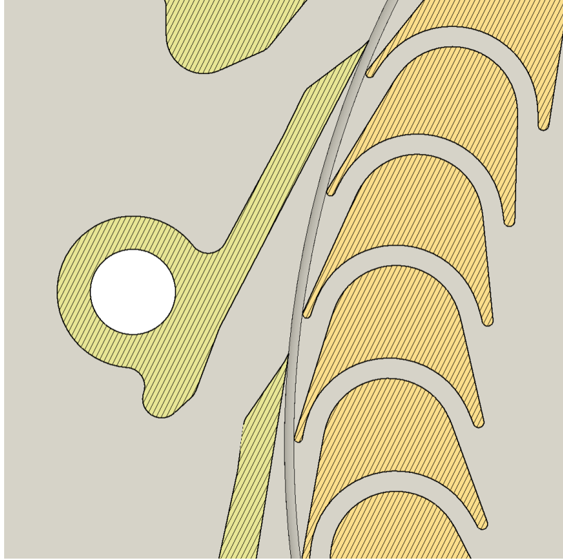
Figure 19: CAD Blade profile
