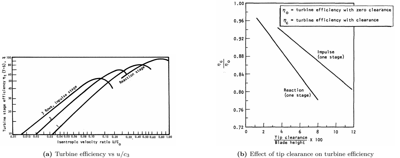
Figure 8: Comparison of efficiency between impulse and reaction turbines against u/c_3 and tip clearance.
