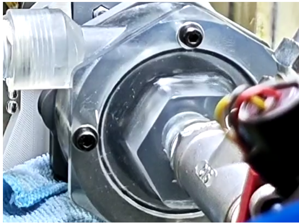
(a) Fully wetted
