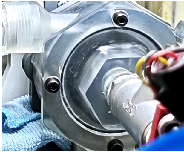
(c) Throat cavitation
