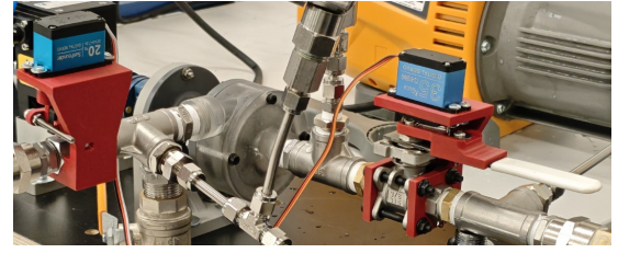
Figure 25: Servo driven throttle valve assembly
