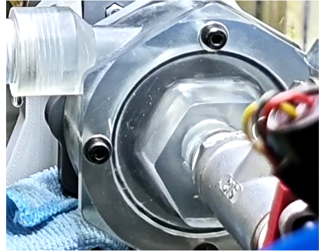
(b) Eye cavitation only
