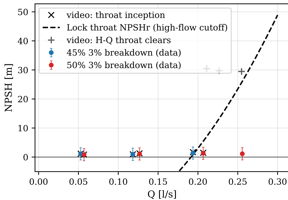
Figure 39: NPSH at 3% head breakdown against flow rate, with the visually observed throat cavitation onsets and the Lock throat cutoff curve. Error bars as in fig. 34.
