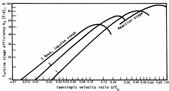
(a) Turbine efficiency vs u/c_3
