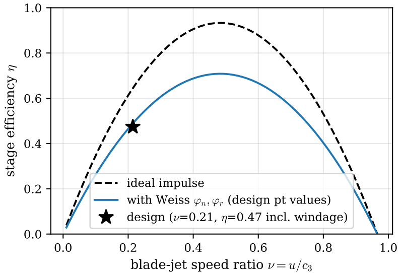
Figure 6: Impulse stage efficiency against blade to jet speed ratio. The dashed line is the ideal impulse stage of eq. (38), the solid line includes the Weiss loss coefficients evaluated at the design point, and the star marks the design point of this turbine, far below the optimum speed ratio.
