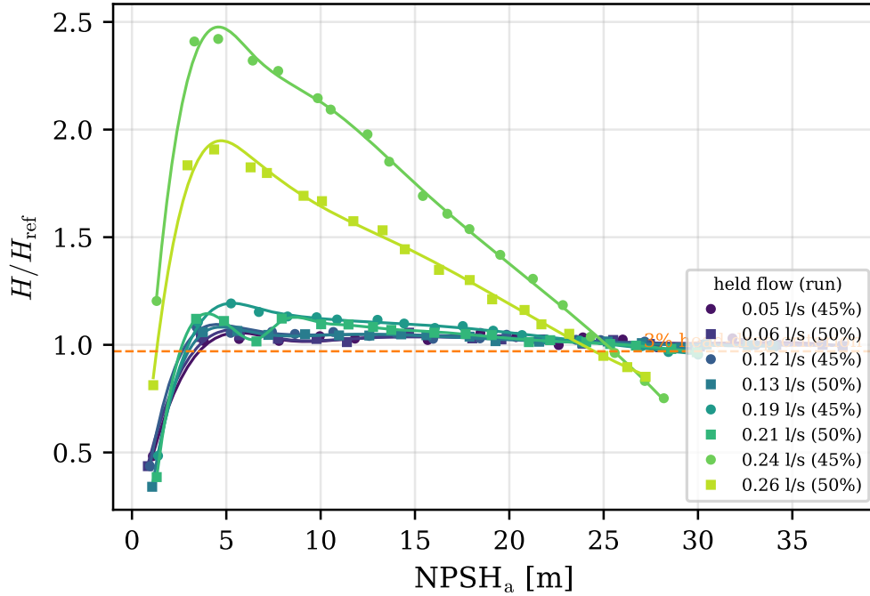
Figure 38: Suction test curves at constant speed: normalised head against NPSH available, one curve per held flow rate, by successive reduction of the inlet pressure. The lines are smoothing splines fitted through them to show the trend. The horizontal line is the 3% head-drop criterion used for fig. 40.
