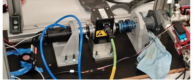
Figure 32: The electric motor and ESC mounted to the test rig.
