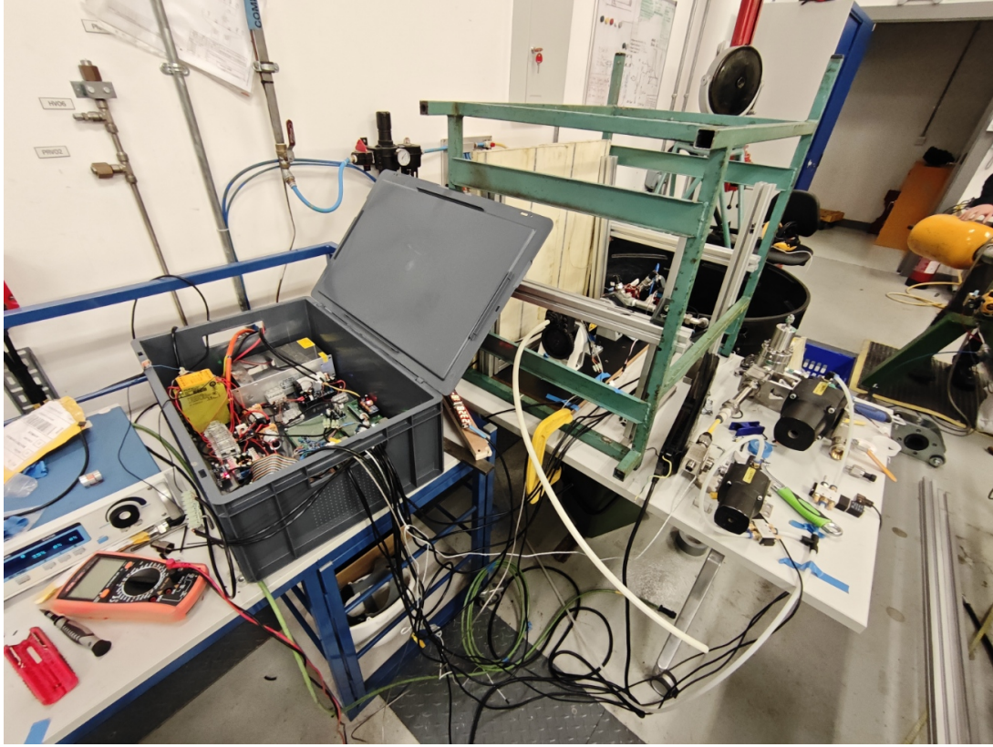
Figure 33: The turbine integrated setup with the pump and the dynamometer.
