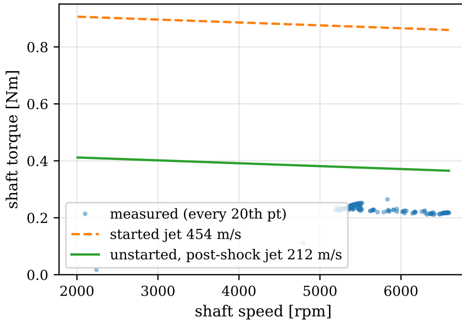
Figure 42: Coupled shaft torque against speed: measured data against the predicted torque lines of eq. (56).
