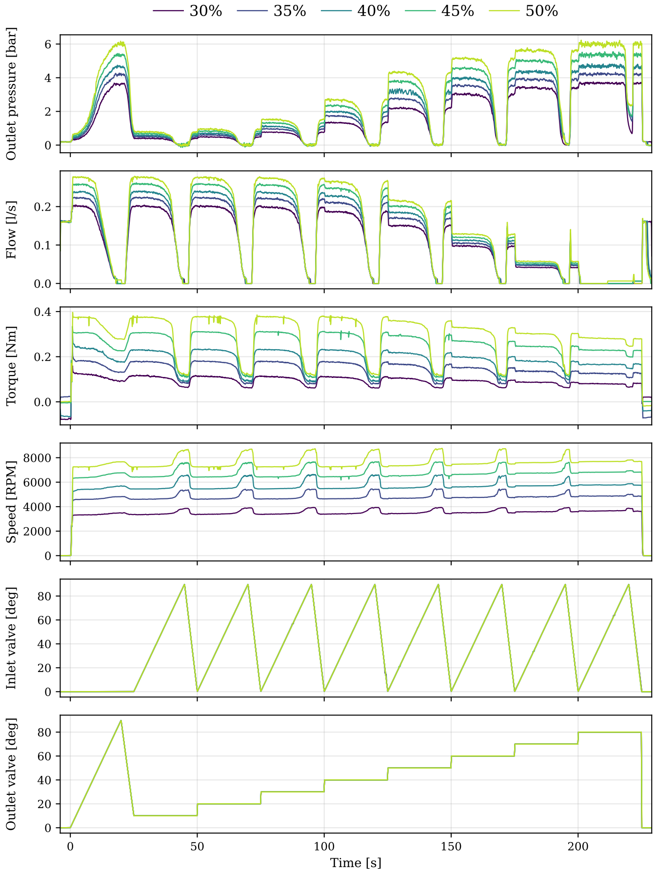
Figure 34: Raw electric pump driven pump experimental data over 5 different motor throttle settings
