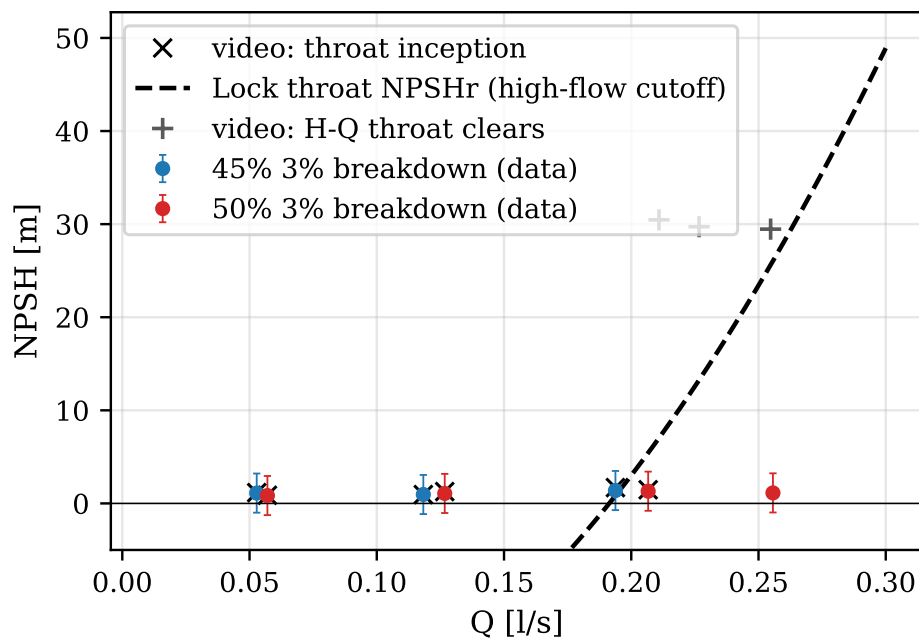
Figure 40: NPSH at 3% head breakdown against flow rate, with the visually observed throat cavitation onsets and the Lock throat cutoff curve. Error bars as in fig. 35.
