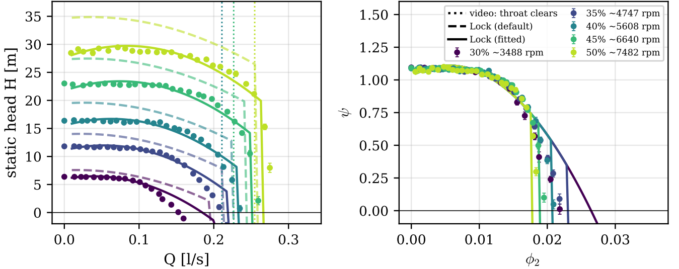
Figure 35: Dimensional and non-dimensional head-flow curves, with two Lock model curves overlayed.
