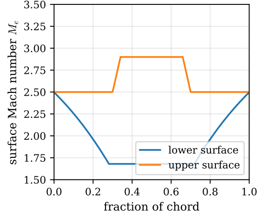
(b) Attempted reproduction of Goldman's distribution of Mach number along the blade surfaces
