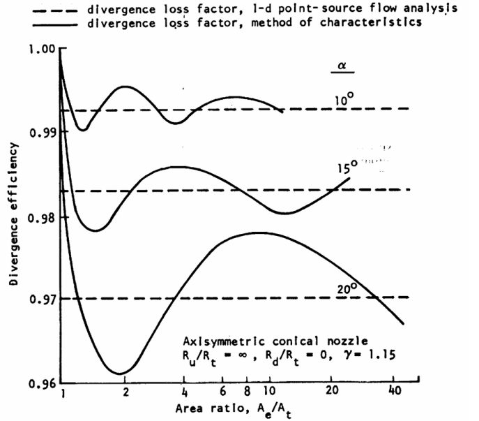
Figure 7. — Variation of theoretical nozzle divergence efficiency with area ratio and divergence half-angle.
