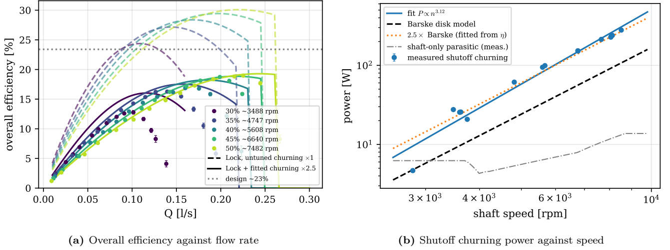
Figure 36: Pump efficiency and the churning measurement.
