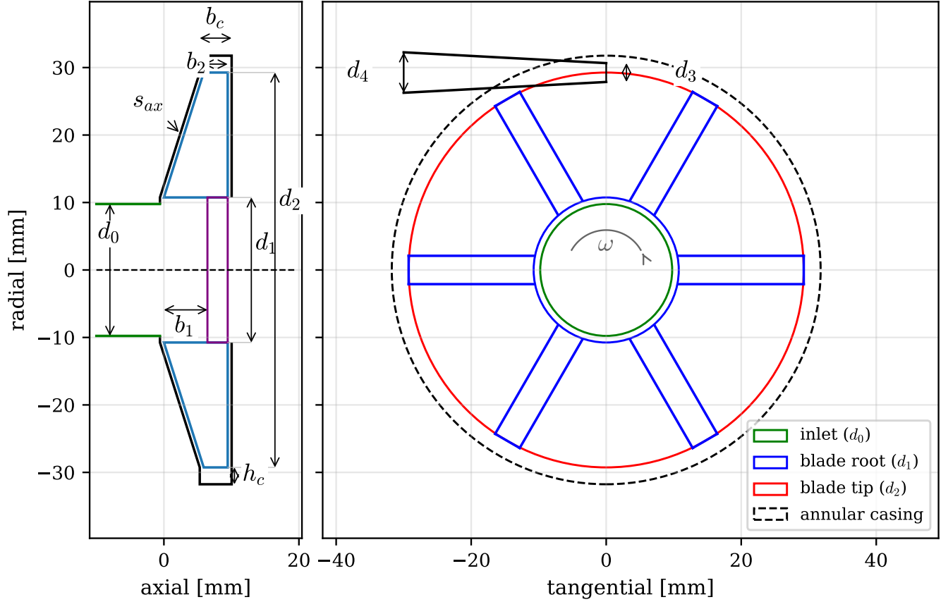
Figure 15: The sized pump geometry, drawn to scale from the sizing code output, with the meridional section (left) and end view (right) sharing the radial axis. The meridional section shows the open tapered blades, the conical front casing maintaining the axial clearance s_{ax} , and the annular casing of width b_c and depth h_c . The end view shows the six radial blades and the single tangential conical diffuser with throat d_3 and exit d_4 . Values are listed in table 2.
