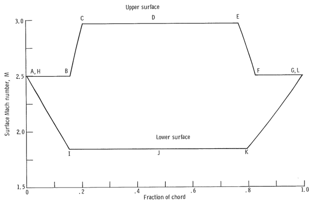
(a) Goldman's published form factor [20]
