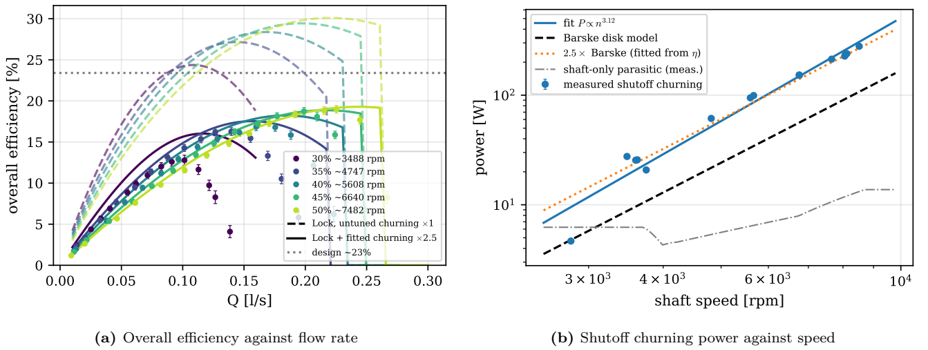
Figure 33: Pump efficiency and the churning measurement. In (a) the dashed curves use Barske’s textbook disc friction and overpredict the efficiency, while the solid curves apply the measured churning multiplier. In (b) the churning power is measured directly at shutoff, where shaft power minus the measured shaft-only parasitic is all churning; the full campaign of 15 shutoff points is used, not just the five canonical runs. Error bars as in fig. 32.
