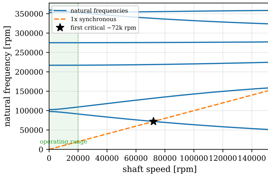
Figure 20: Campbell diagram of the turbine shaft from a finite element rotor model (10 mm solid aluminium shaft, turbine disk overhung, ball bearing stiffness; the coupler side disk is omitted). The first bending pair starts near 99,000 RPM at standstill and the backward whirl branch crosses the synchronous line at around 72,000 RPM, leaving a margin of more than 3.5 over the operating range.
