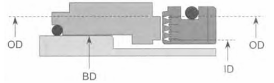
Figure 16: Geometric dimensions of an OD pressurized the mechanical seal by Karrasik [4].
