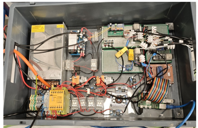
Figure 28: The electronics box with the Raspberry Pi, ESP32S3s and power supply.
