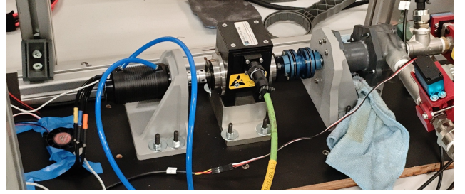
Figure 31: The electric motor and ESC mounted to the test rig.
