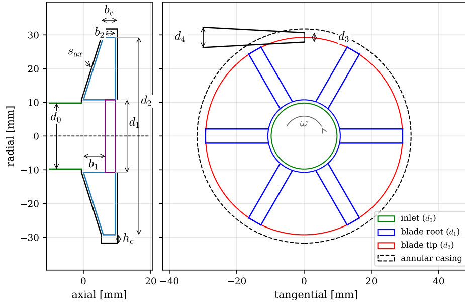
Figure 14: The sized pump geometry drawn to scale. The meridional section (left) and plan view (right).
