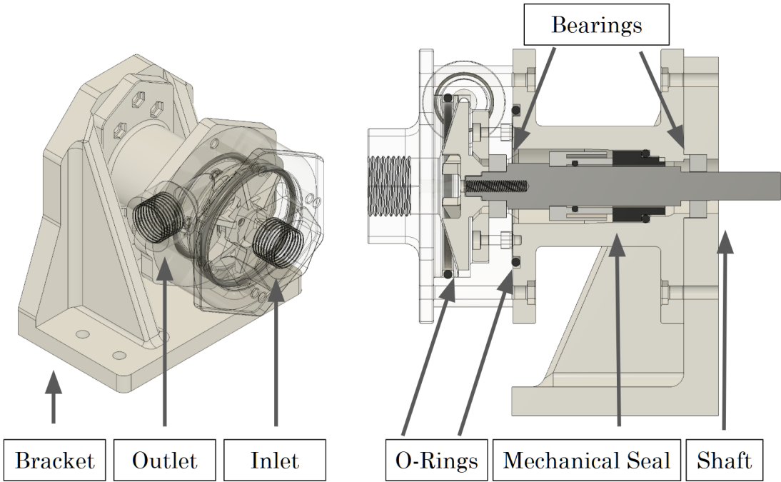
Figure 15: Labeled CAD isotropic and section view of the pump assembly
