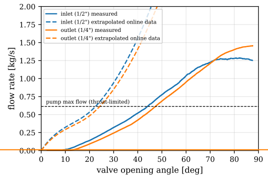
Figure 25: Extrapolated against measured valve capacity
