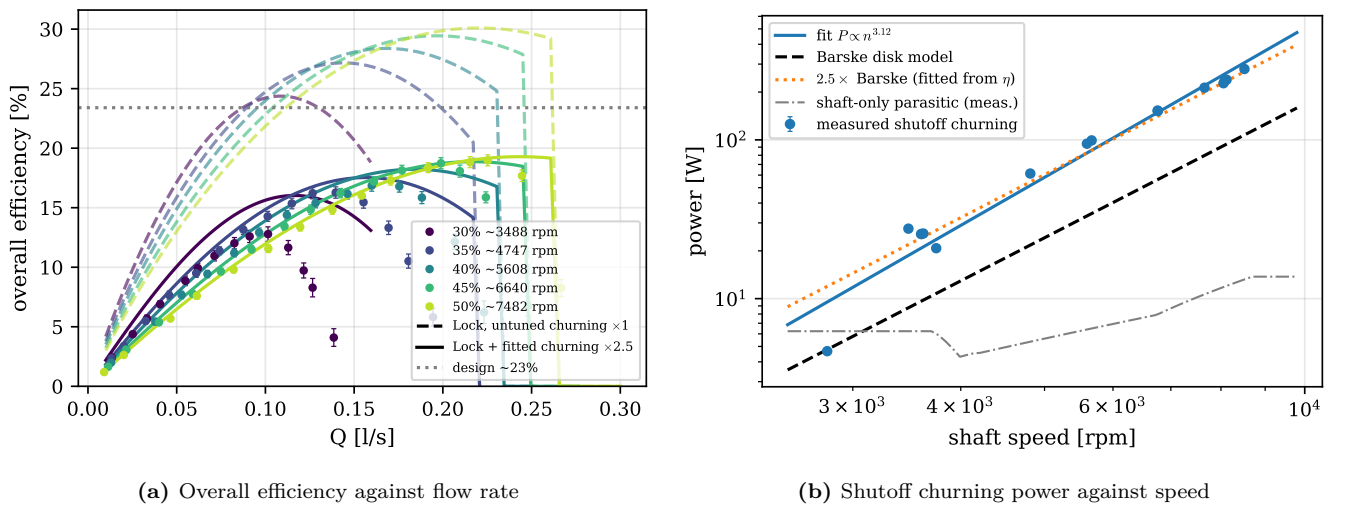
Figure 32: Pump efficiency and the churning measurement. In (a) the dashed curves use Barske’s textbook disc friction and overpredict the efficiency, while the solid curves apply the measured churning multiplier. In (b) the churning power is measured directly at shutoff, where shaft power minus the measured shaft-only parasitic is all churning; the full campaign of 15 shutoff points is used, not just the five canonical runs. Error bars as in fig. 31.
