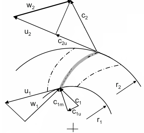
Figure 2: Velocity triangles in a conventional pump, adapted from Gülich
