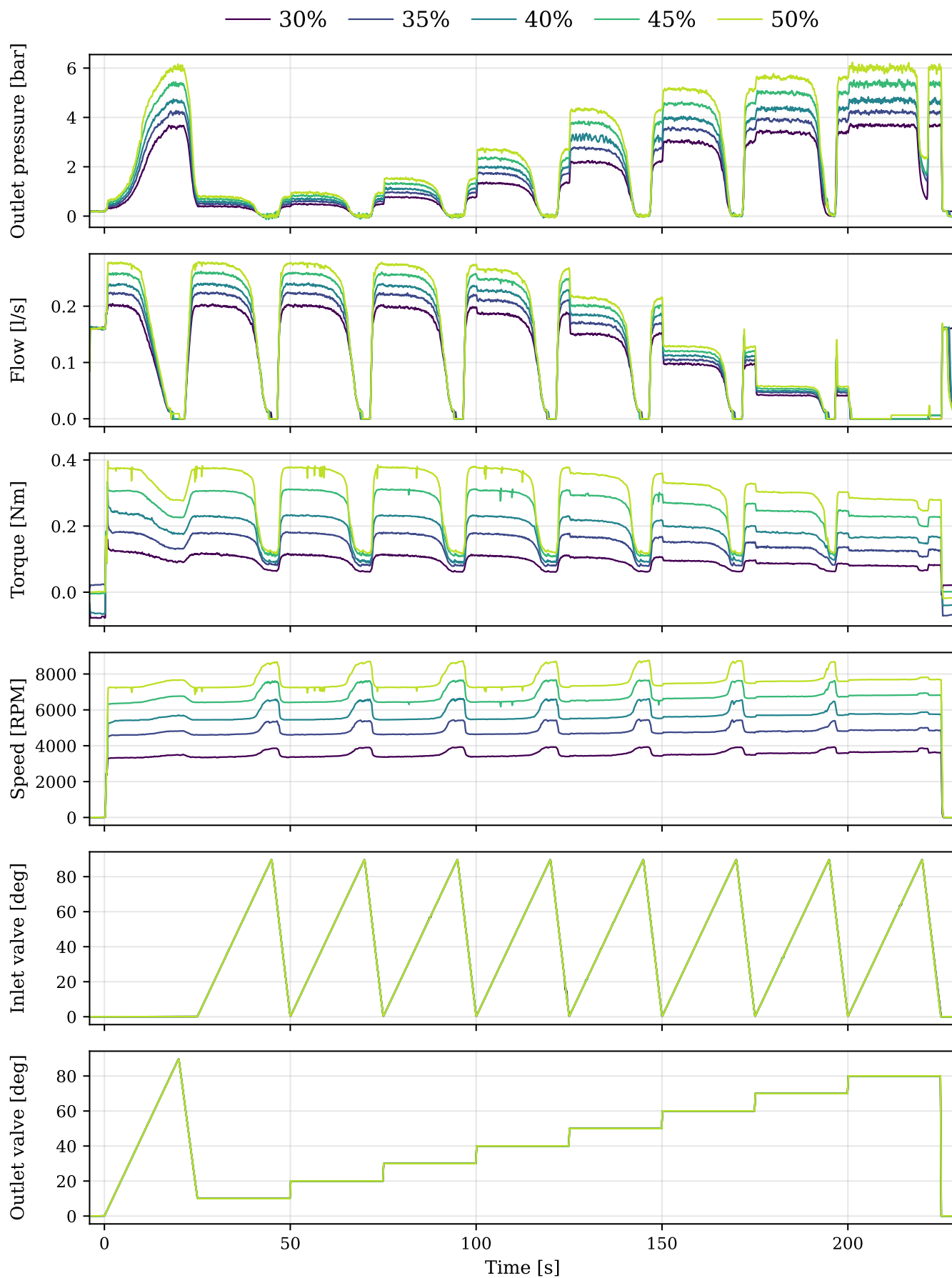
Figure 33: Raw electric pump driven pump experimental data over 5 different motor throttle settings
