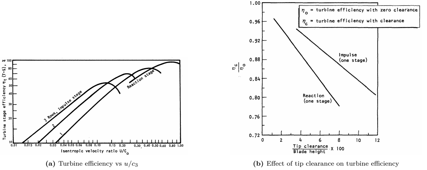
Figure 8: Comparison of efficiency between impulse and reaction turbines against u/c_3 and tip clearance.
