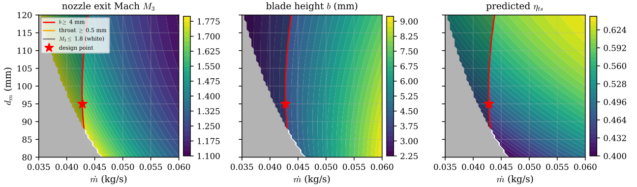
Figure 18: The turbine design space over mean diameter and mass flow, evaluated with the full sizing and loss model at the design speed. The panels show nozzle exit Mach number, blade height and predicted total to static efficiency. Overlaid lines are the design constraints (blade height \geq 4 mm, nozzle throat \geq 0.5 mm, M_3 \leq 1.8 ), the shaded region is infeasible, and the marker is the selected design point.
