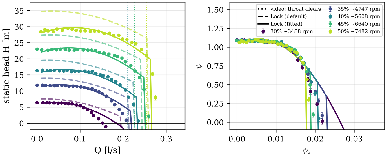
Figure 34: Dimensional and non-dimensional head-flow curves, with two Lock model curves overlayed.
