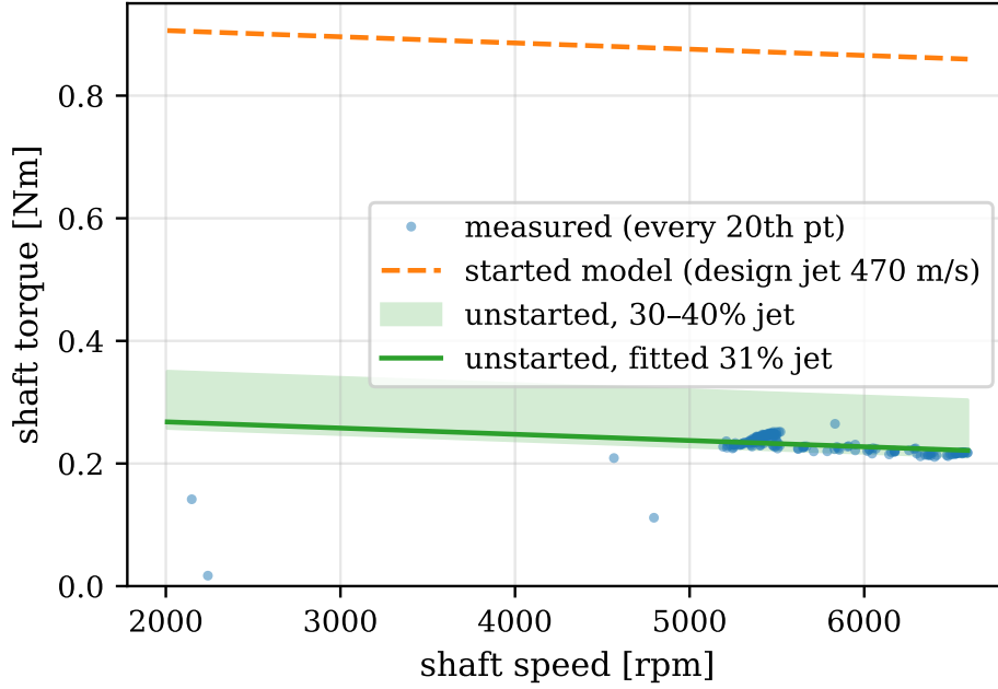
Figure 42: Coupled shaft torque against speed: measured data, the started flow model (dashed) and the unstarted model with a reduced effective jet (solid with band). The factor of four deficit against the started model is explained by the rotor running unstarted below the starting threshold.
