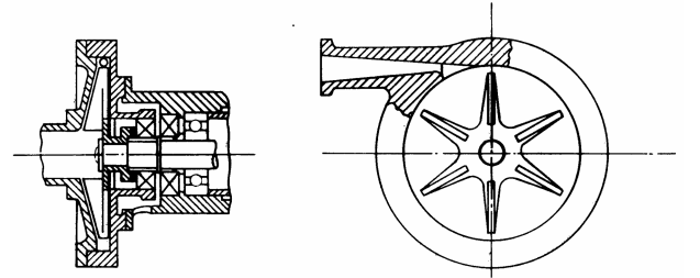
(b) Barske open partial emission impeller
