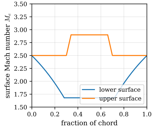
(b) Attempted reproduction of Goldman's distribution of Mach number along the blade surfaces
