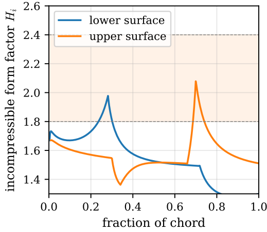
(a) Attempted reproduction of Goldman's incompressible form factor H_i along the blade surfaces
