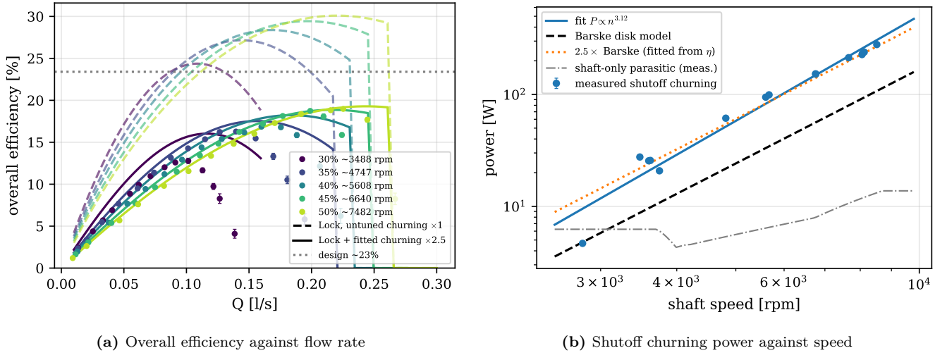
Figure 35: Pump efficiency and the churning measurement. In (a) the dashed curves use Barske's textbook disc friction and overpredict the efficiency, while the solid curves apply the measured churning multiplier. In (b) the churning power is measured directly at shutoff, where shaft power minus the measured shaft-only parasitic is all churning; the full campaign of 15 shutoff points is used, not just the five canonical runs. Error bars as in fig. 34.
