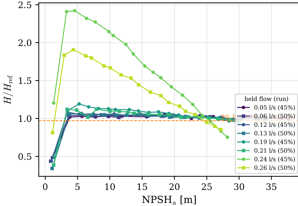
Figure 39: Suction test curves at constant speed: normalised head against NPSH available, one curve per held flow rate, by successive reduction of the inlet pressure. The horizontal line is the 3% head-drop criterion used for fig. 38.
