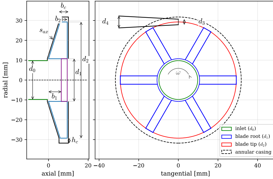
Figure 15: The sized pump geometry drawn to scale. The meridional section (left) and plan view (right).
