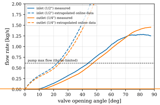
Figure 26: Extrapolated against measured valve capacity
