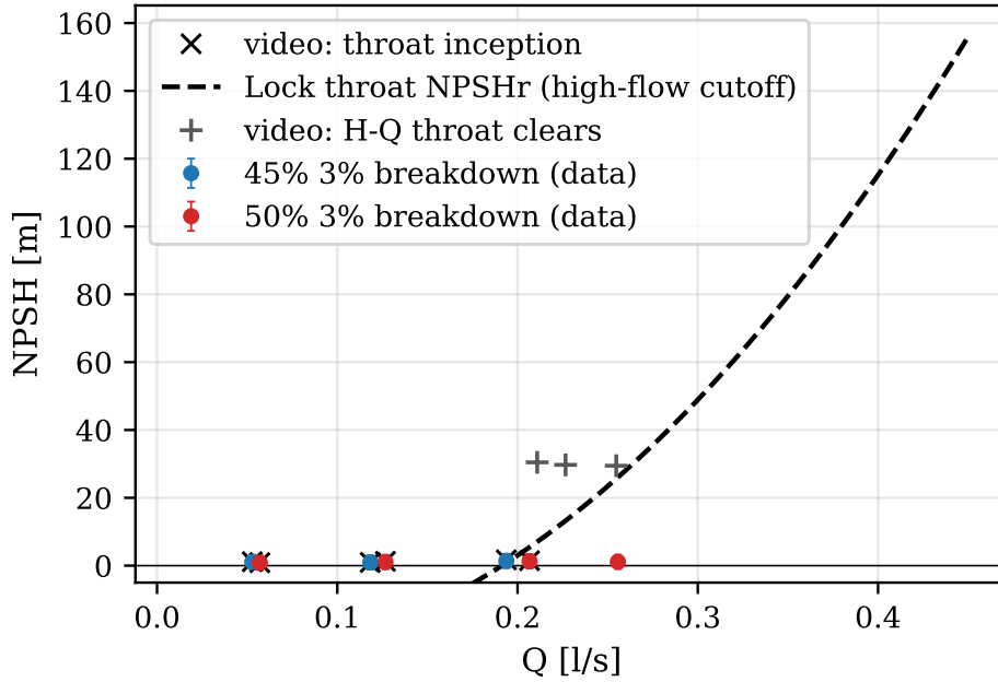
Figure 38: NPSH at 3% head breakdown against flow rate, with the visually observed throat cavitation onsets and the Lock throat cutoff curve. Error bars as in fig. 34.
