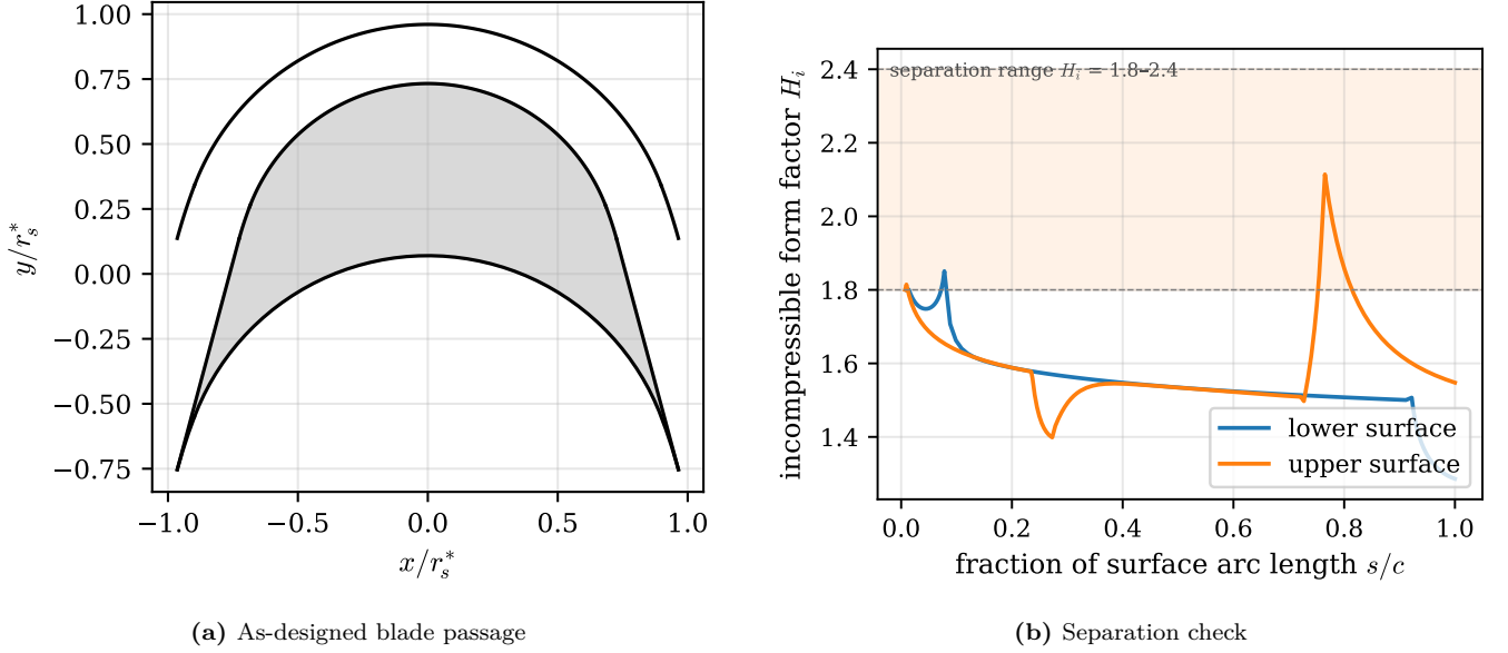
Figure 19: The ideal MoC countour and incompressible form factor H_i check for the design surface mach numbers M_l = 1.05 and M_u = 1.5 .
