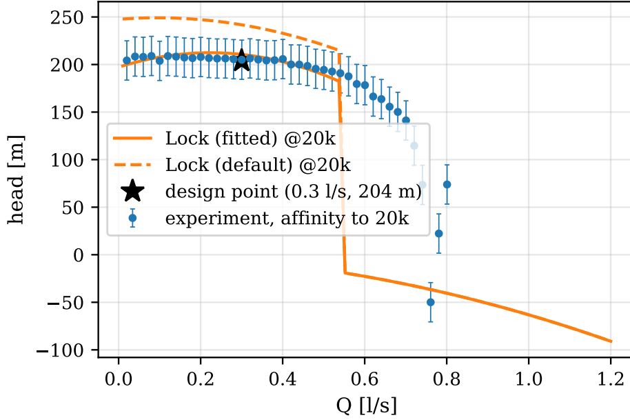
Figure 43: The pooled non dimensional characteristic carried to 20000 rpm by the affinity laws, with the Lock model at design speed and the design point marked.
