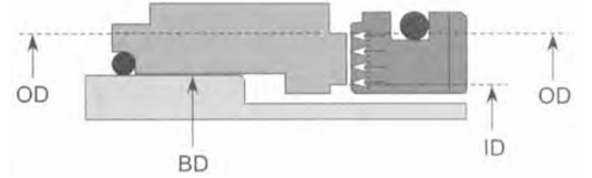
Figure 17: Geometric dimensions of an OD pressurized the mechanical seal by Karassik [4].
