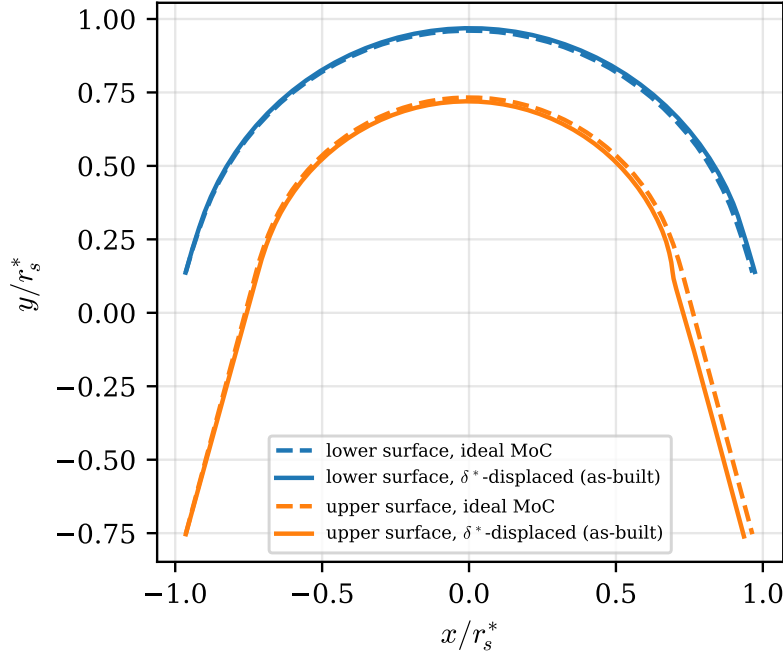
Figure 20: Ideal MoC contour (dashed) against the boundary layer displaced contour that was actually manufactured (solid). The surfaces are offset by the local displacement thickness \delta^* from the Sasman and Cresci solution, so that the printed passage presents the inviscid design geometry to the core flow.
