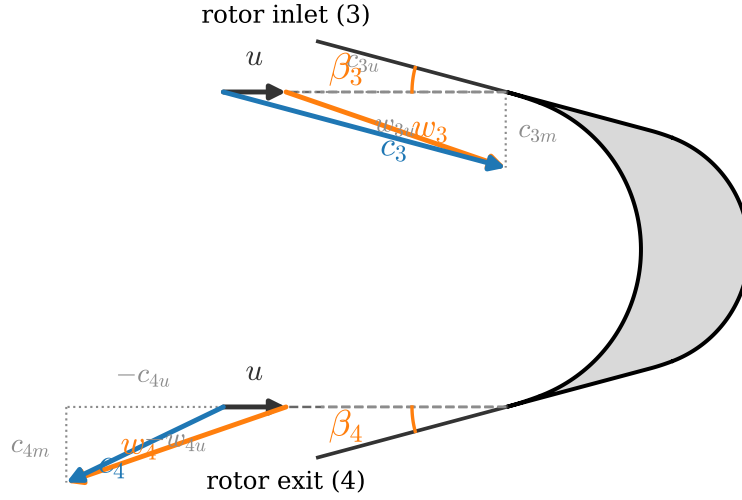
Figure 5: Impulse turbine velocity triangle nomenclature at the rotor inlet (station 3) and exit (station 4). The design point triangles with actual values are shown in fig. 16.
