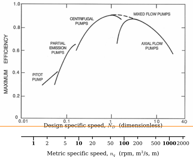
Figure 1: Optimum pump geometry and attainable efficiency against specific speed. Adapted from Balje [1] with specific speed in n_q units.
