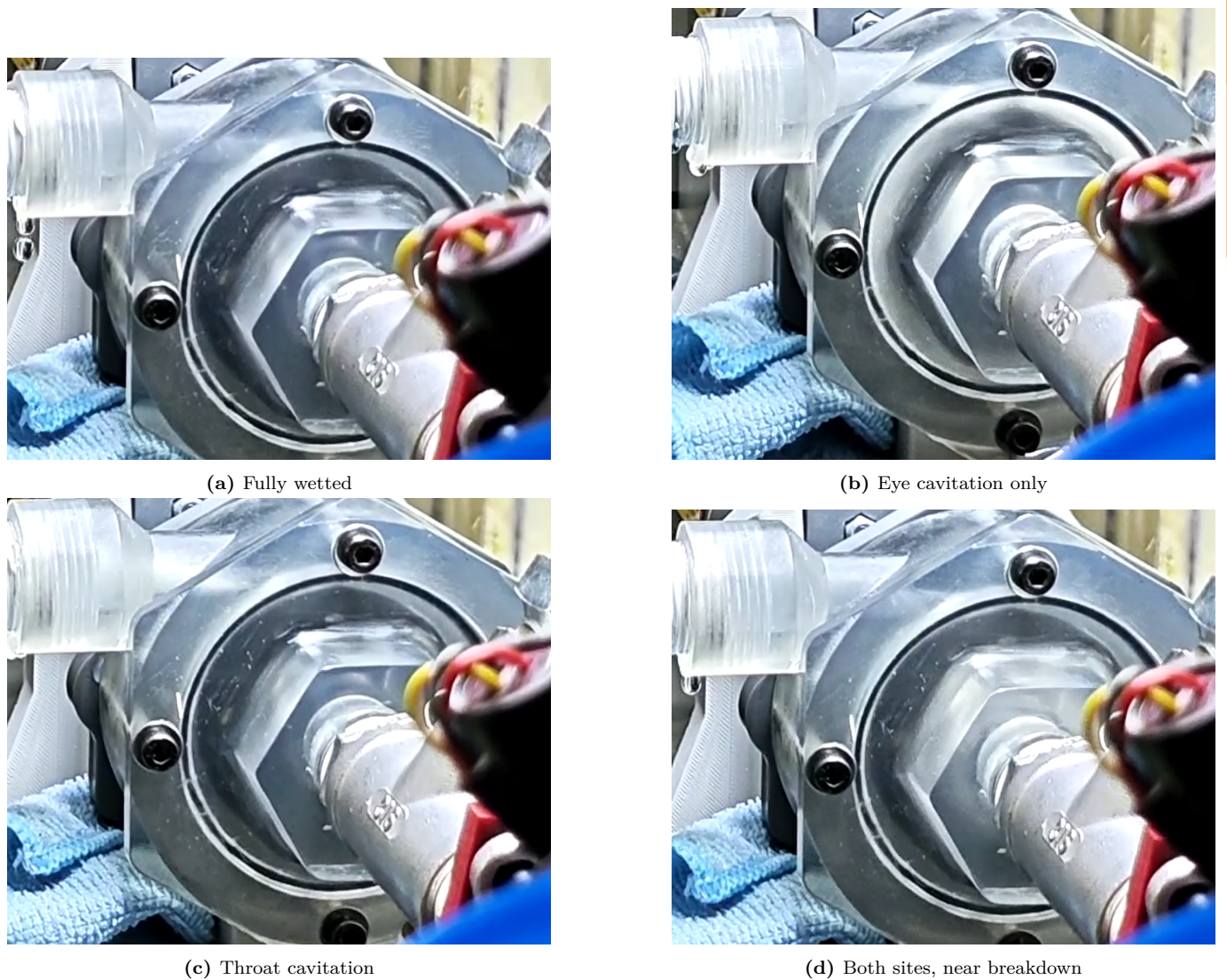
Figure 39: Stills through the transparent front casing at descending NPSH. The eye cavitates first with no measurable head effect, while the appearance of throat cavitation coincides with the head breakdown. Frame timestamps are synchronised to the logged data.
