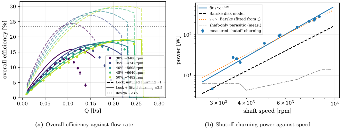
Figure 35: Pump efficiency and the churning measurement.
