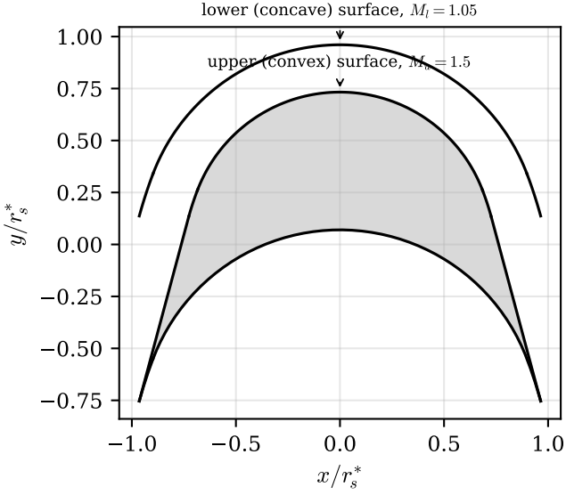
(a) As-designed blade passage
