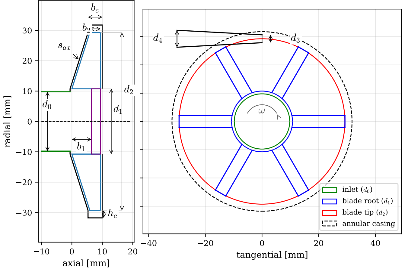
Figure 12: The sized pump geometry, drawn to scale from the sizing code output, with the meridional section (left) and end view (right) sharing the radial axis. The meridional section shows the open tapered blades, the conical front casing maintaining the axial clearance s_{ax} , and the annular casing of width b_c and depth h_c . The end view shows the six radial blades and the single tangential conical diffuser with throat d_3 and exit d_4 . Values are listed in table 2.
