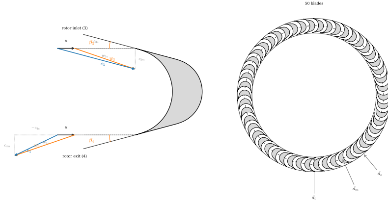
Figure 5: Impulse turbine velocity triangle nomenclature at the rotor inlet (station 3) and exit (station 4). The design point triangles with actual values are shown in fig. 16.
