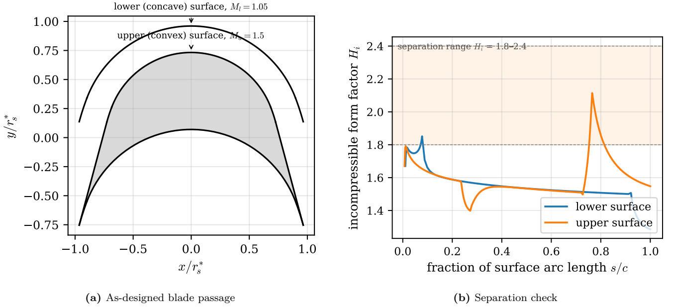
Figure 18: The as-designed MoC blade passage and its separation check. The form factor H_i is evaluated on both surfaces at the design point inlet conditions and touches 2.1 at around 77% chord on the upper surface, at the bottom of the 1.8 to 2.4 separation band. The blade is separation imminent by design, which per Goldman is where the efficiency optimum sits.
