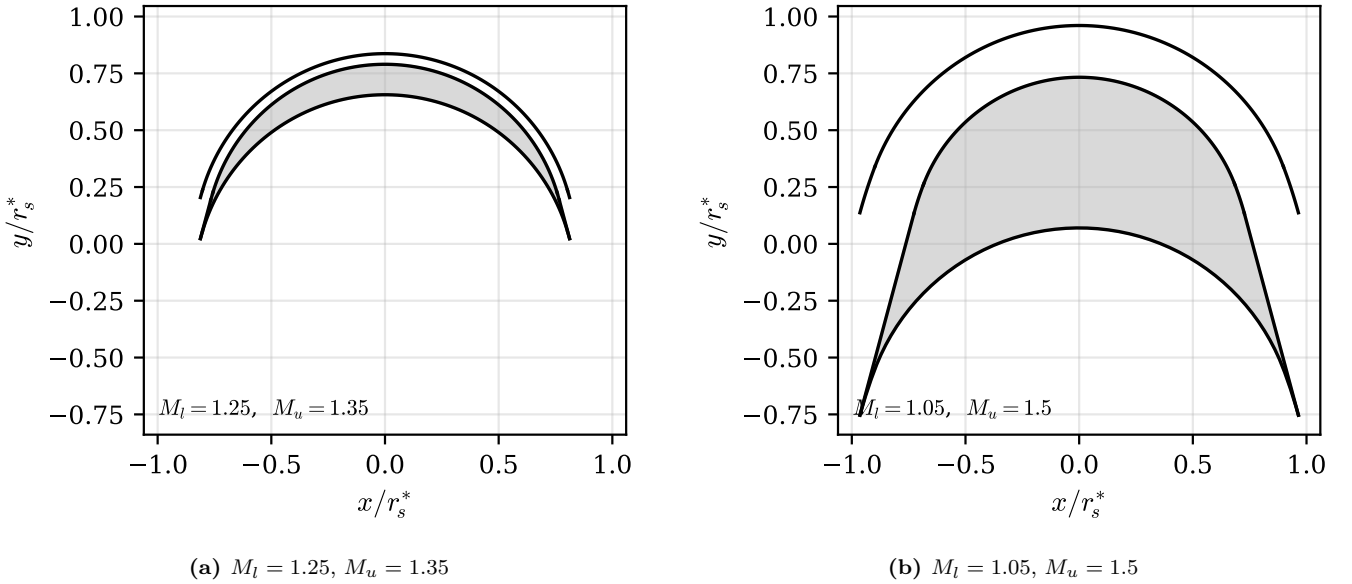
Figure 10: The effect of surface Mach number spread on the blade passage, for the same inlet conditions and shared axis scales. A narrow spread produces a sliver of a passage where the boundary layers occupy a large fraction of the width, while a wide spread opens the passage up. This is why efficiency rises with Mach spread until separation or starting limits are hit.
