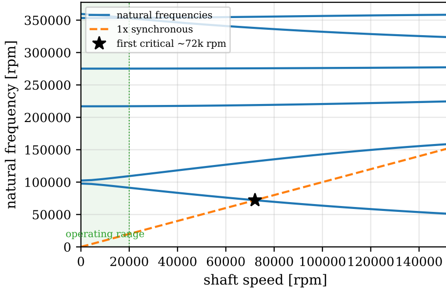
Figure 21: Campbell diagram of the turbine shaft from a finite element rotor model (10 mm solid aluminium shaft, turbine disk overhung, ball bearing stiffness; the coupler side disk is omitted). The first bending pair starts near 99,000 RPM at standstill and the backward whirl branch crosses the synchronous line at around 72,000 RPM, leaving a margin of more than 3.5 over the operating range.
