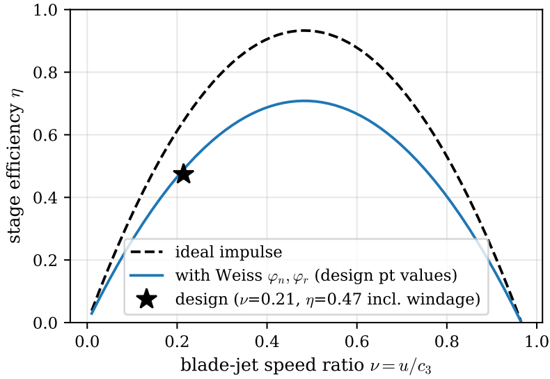
Figure 8: Impulse stage efficiency against blade to jet speed ratio. The dashed line is the ideal impulse stage of eq. (35), the solid line includes the Weiss loss coefficients evaluated at the design point, and the star marks the design point of this turbine, far below the optimum speed ratio.
