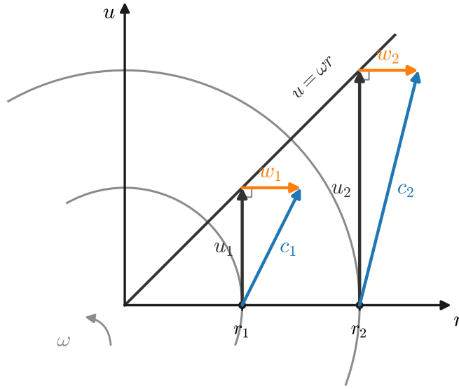
Figure 4: Velocity triangle nomenclature and the forced vortex flow field in the Barske impeller, where the fluid rotates as a solid body so the tangential velocity equals the local blade speed, u = \omega r .
