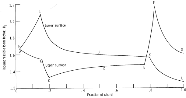
(a) Goldman's published distribution [16]
