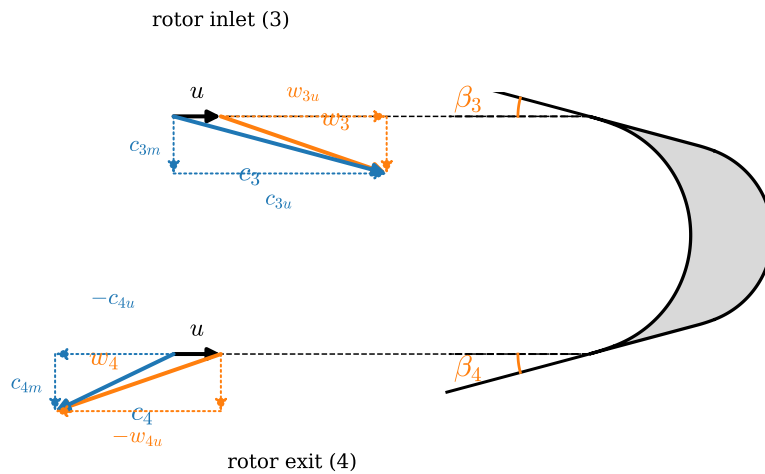
Figure 5: Impulse turbine velocity triangle nomenclature at the rotor inlet (station 3) and exit (station 4). The design point triangles with actual values are shown in fig. 16.
