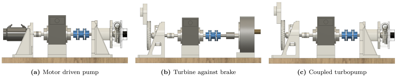
Figure 21: The three test configurations. In each case the TM306 torquemeter sits between the driving component and the load, so torque is measured at the shaft.
