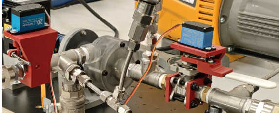
(a) Servo driven throttle valve assembly
