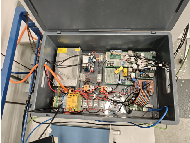
(a) The electronics box with the Raspberry Pi, ESP32S3s and power supply.
