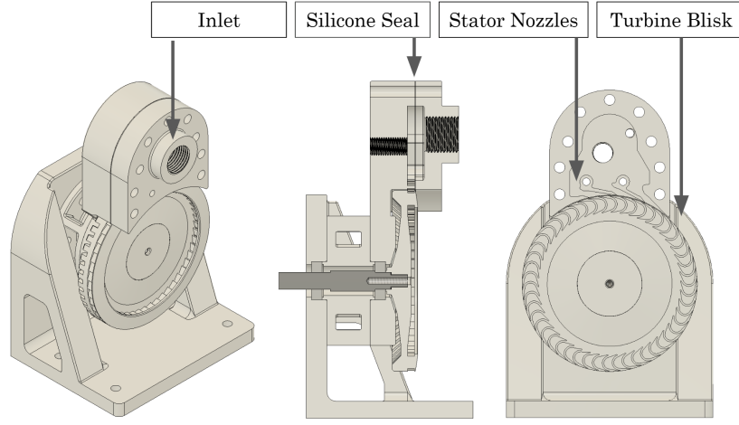
Figure 20: Labeled CAD isotropic and section view of the turbine assembly
