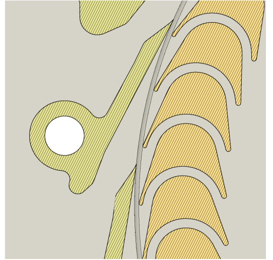
Figure 19: CAD Blade profile
