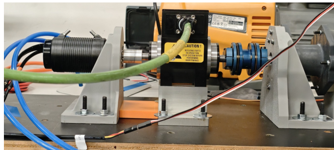
Figure 22: Shaft alignment procedure using the flat faces of the component mounts.
