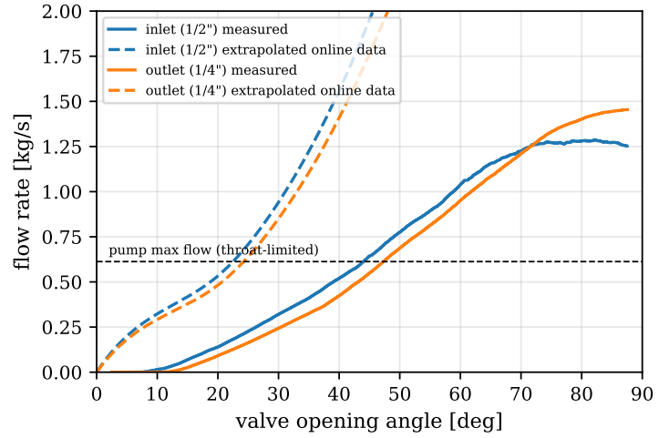
(b) Extrapolated against measured valve capacity
