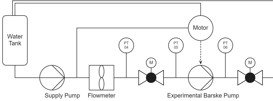
Figure 23: P&ID of the water circuit for the electric motor driven pump test configuration.
