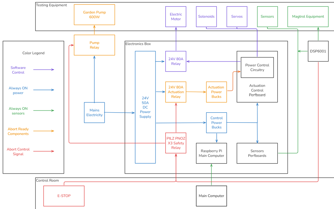
Figure 26: Block diagram of full electronics system including safety, data acquisition, and control components.
