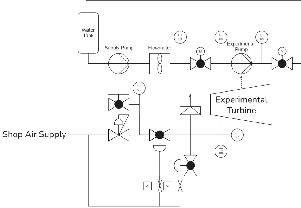
Figure 25: P&ID of the water and air circuit for the turbopump configuration.
