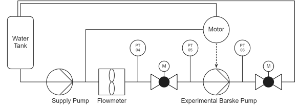
Figure 23: P&ID of the water circuit for the electric motor driven pump test configuration.
