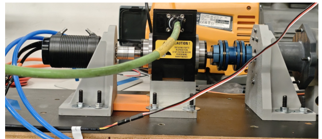
Figure 22: Shaft alignment procedure using the flat faces of the component mounts.
