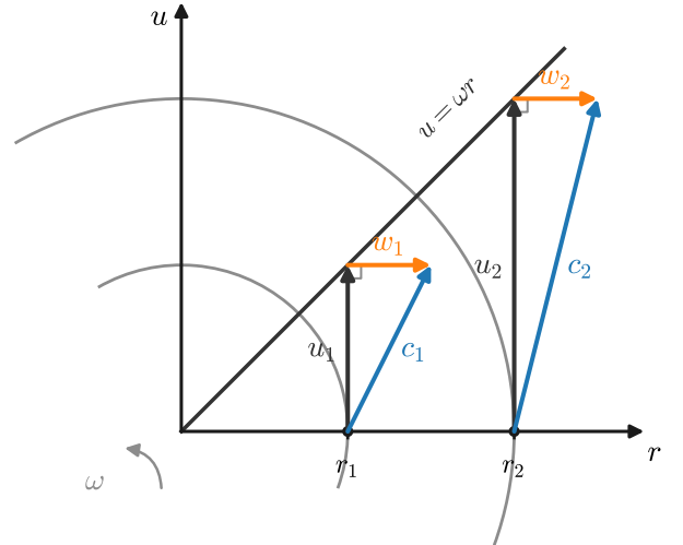
Figure 6: Velocity triangles in a forced vortex pump
