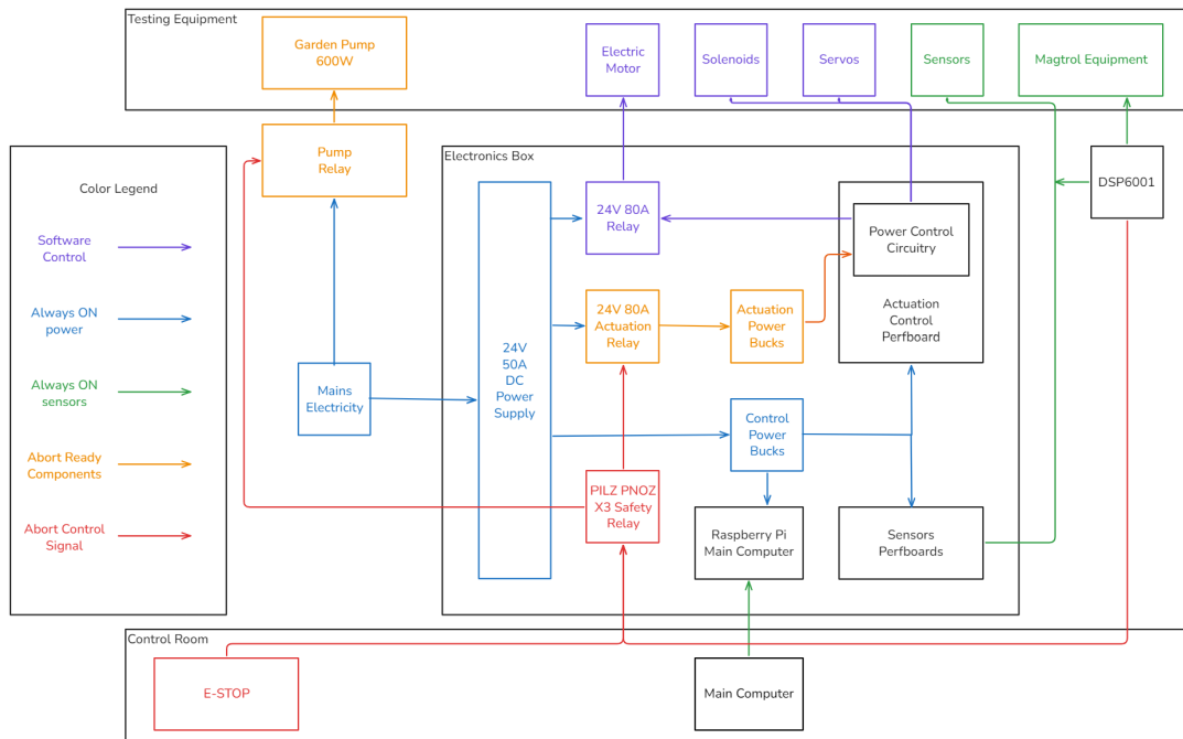
Figure 27: Block diagram of full electronics system including safety, data acquisition, and control components.
