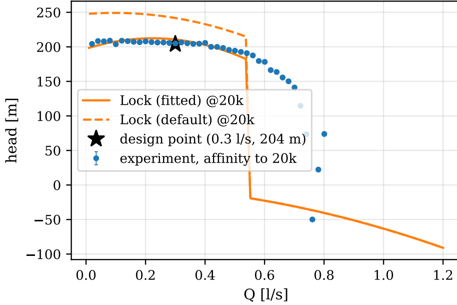
Figure 40: The pooled non dimensional characteristic carried to 20000 rpm by the affinity laws, with the Lock model at design speed and the design point marked.
