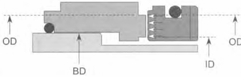
Figure 16: Geometric dimensions of an OD pressurized the mechanical seal by Karrasik [4].
