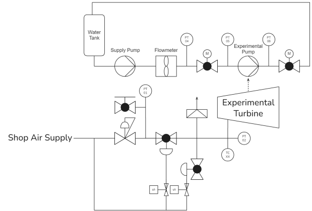
Figure 26: P&ID of the water and air circuit for the turbopump configuration.
