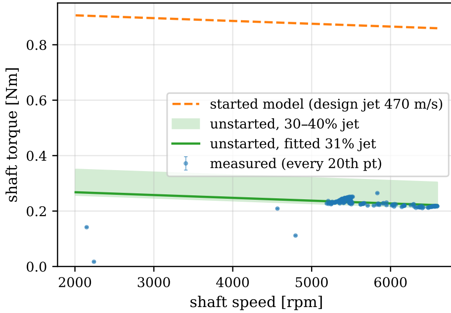
Figure 39: Coupled shaft torque against speed: measured data, the started flow model (dashed) and the unstarted model with a reduced effective jet (solid with band). The factor of four deficit against the started model is explained by the rotor running unstarted below the starting threshold.
