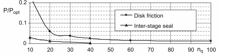
Figure 3: Disc friction loss vs specific speed n_q after Gülich. At low specific speed the disc friction dominates.
