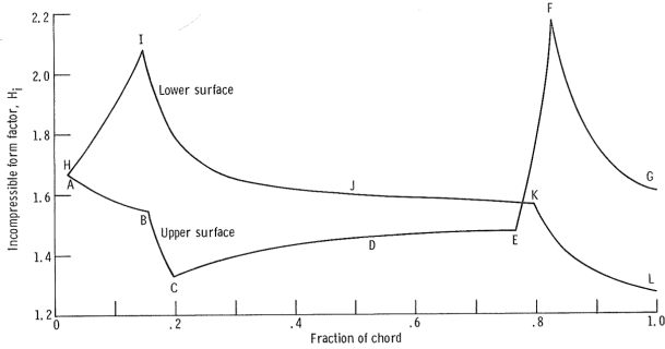
(a) Goldman's published distribution [19]
