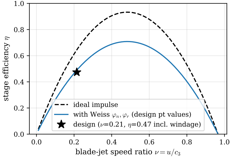
Figure 8: Impulse stage efficiency against blade to jet speed ratio. The dashed line is the ideal impulse stage of eq. (30), the solid line includes the Weiss loss coefficients evaluated at the design point, and the star marks the design point of this turbine, far below the optimum speed ratio.
