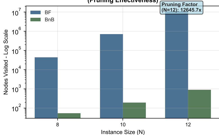
Nodes Visited Comparison (Pruning Effectiveness)
