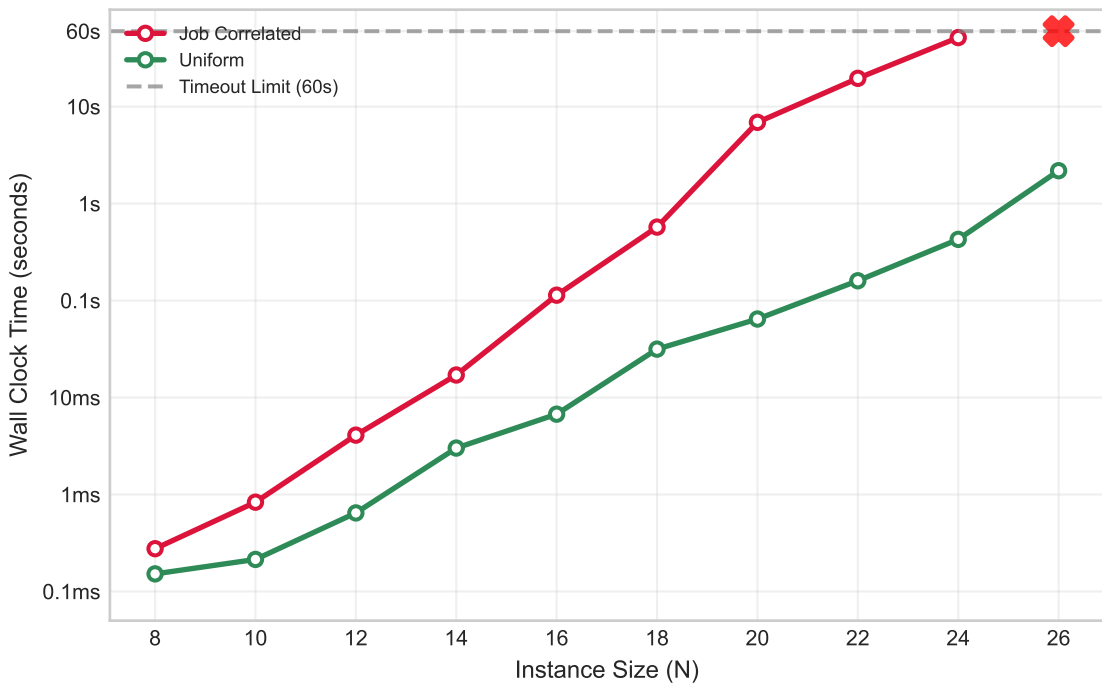
Pilot A: Branch & Bound "The Wall" (M=4)
