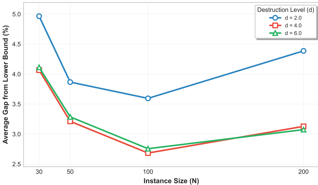
Parameter Interaction Effects (Instance Size vs Gap by Destruction Level)
