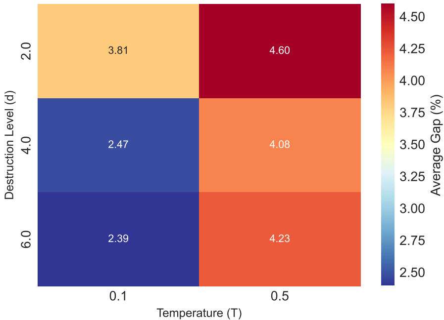
Parameter Tuning Heatmap (Lower is Better)
