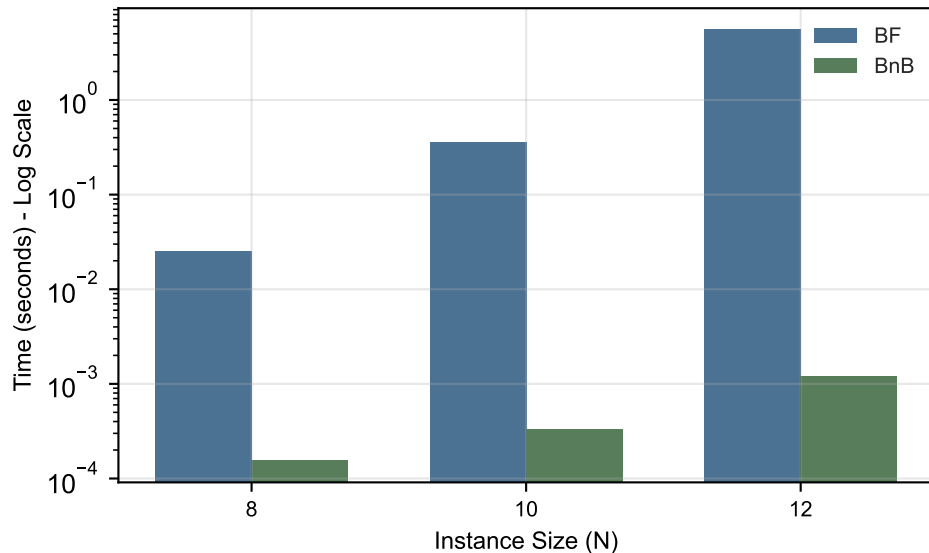
Execution Time Comparison (Brute Force vs Branch & Bound)
