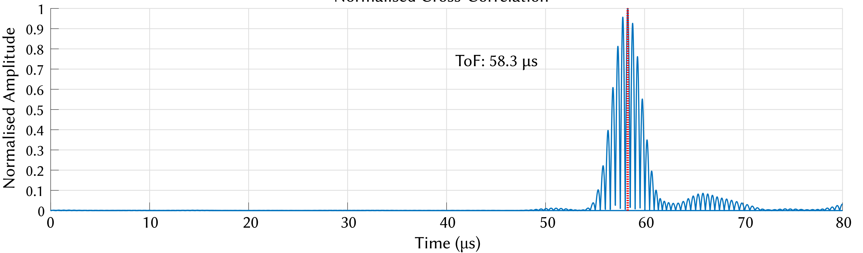
Normalised Cross-Correlation
