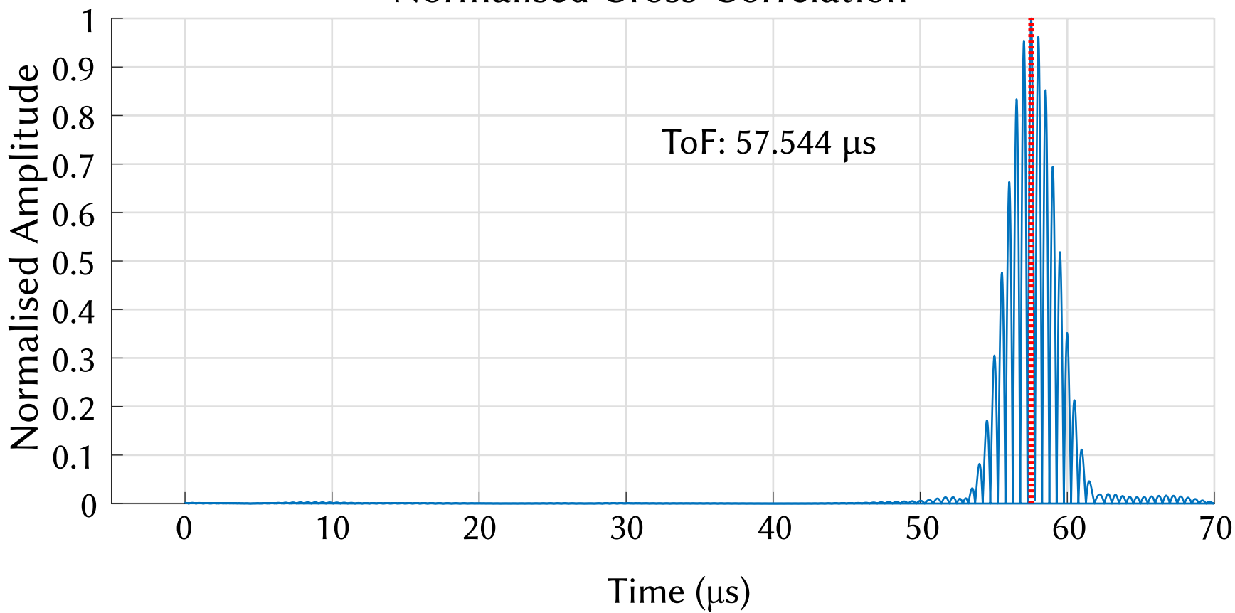
Normalised Cross-Correlation
