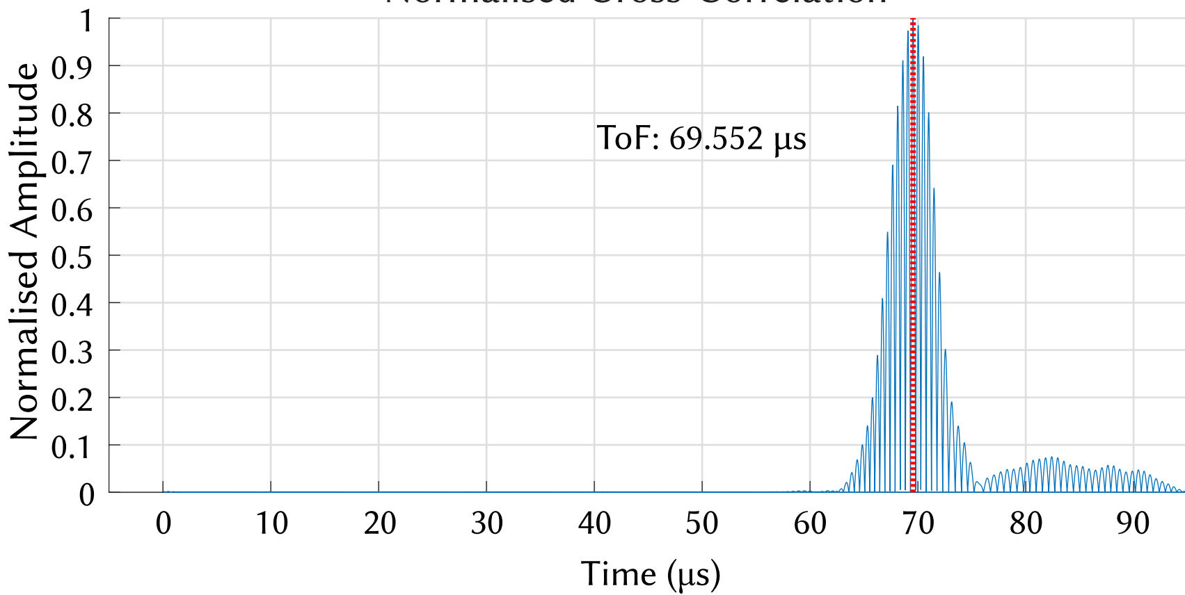
Normalised Cross-Correlation
