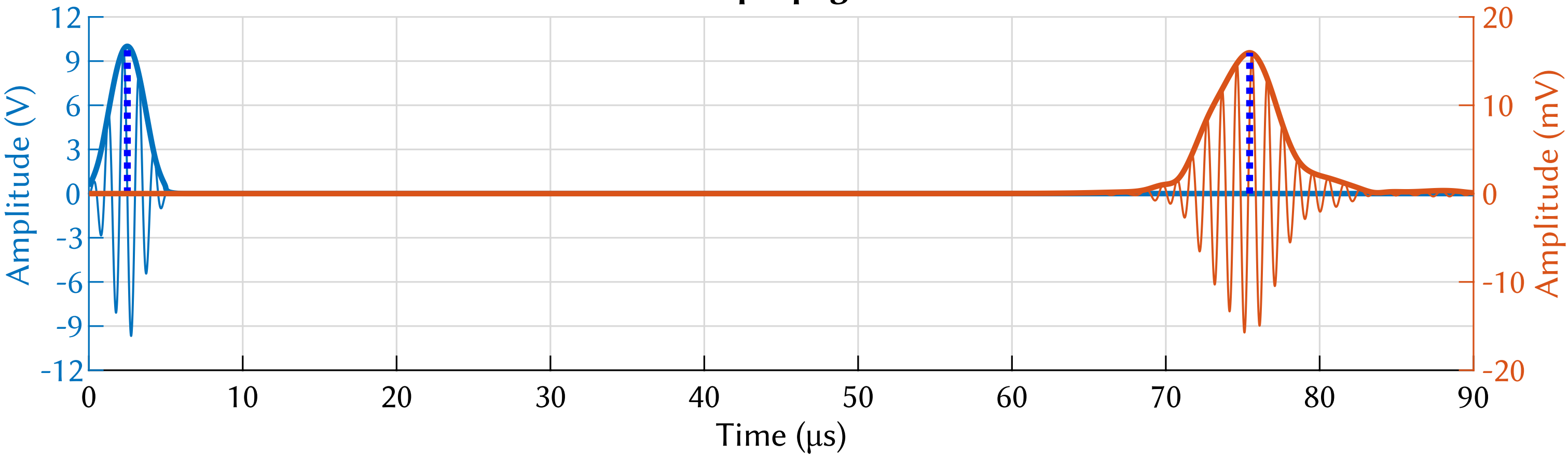
A1 mode wave propagation at 100°C
