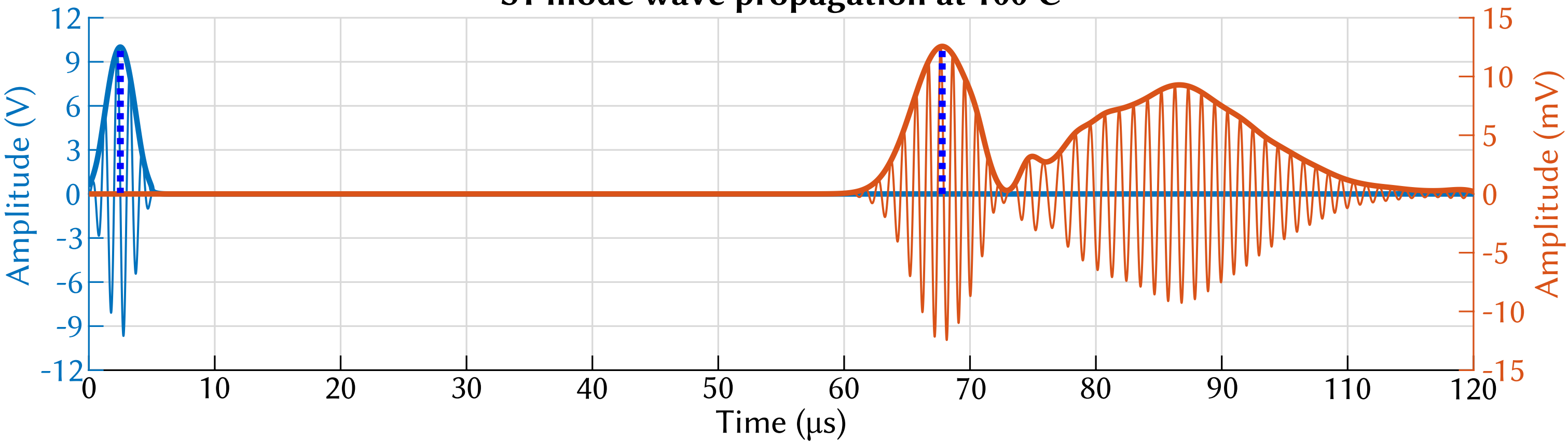
S1 mode wave propagation at 100°C
