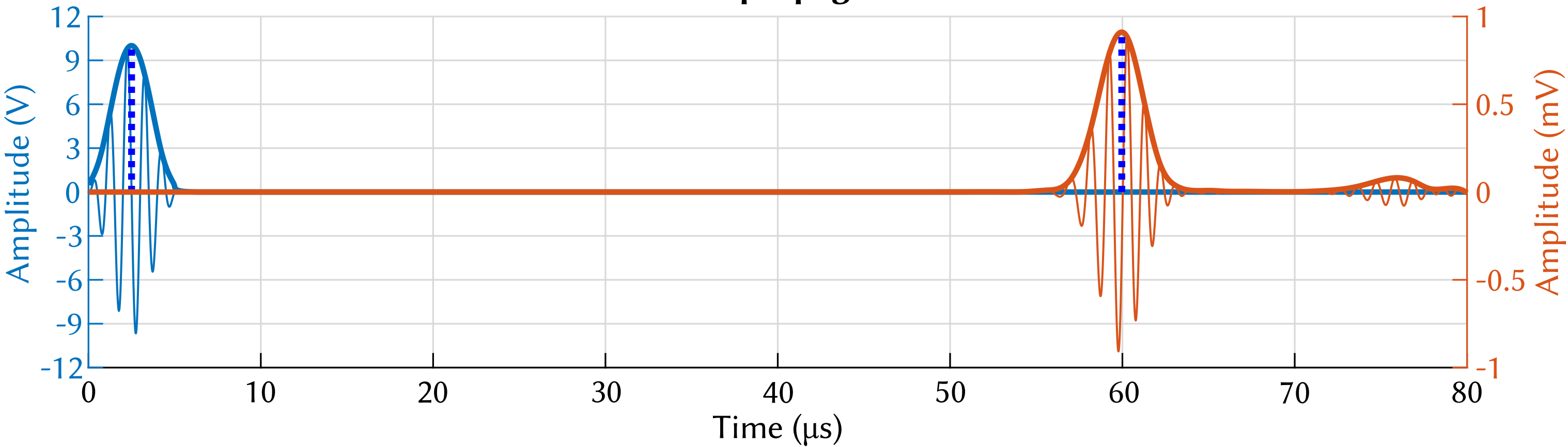
S0 mode wave propagation at 100°C
