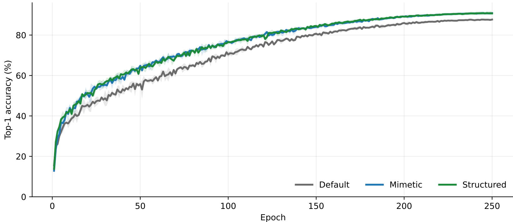
CIFAR-10 Seed Stability Across Training
