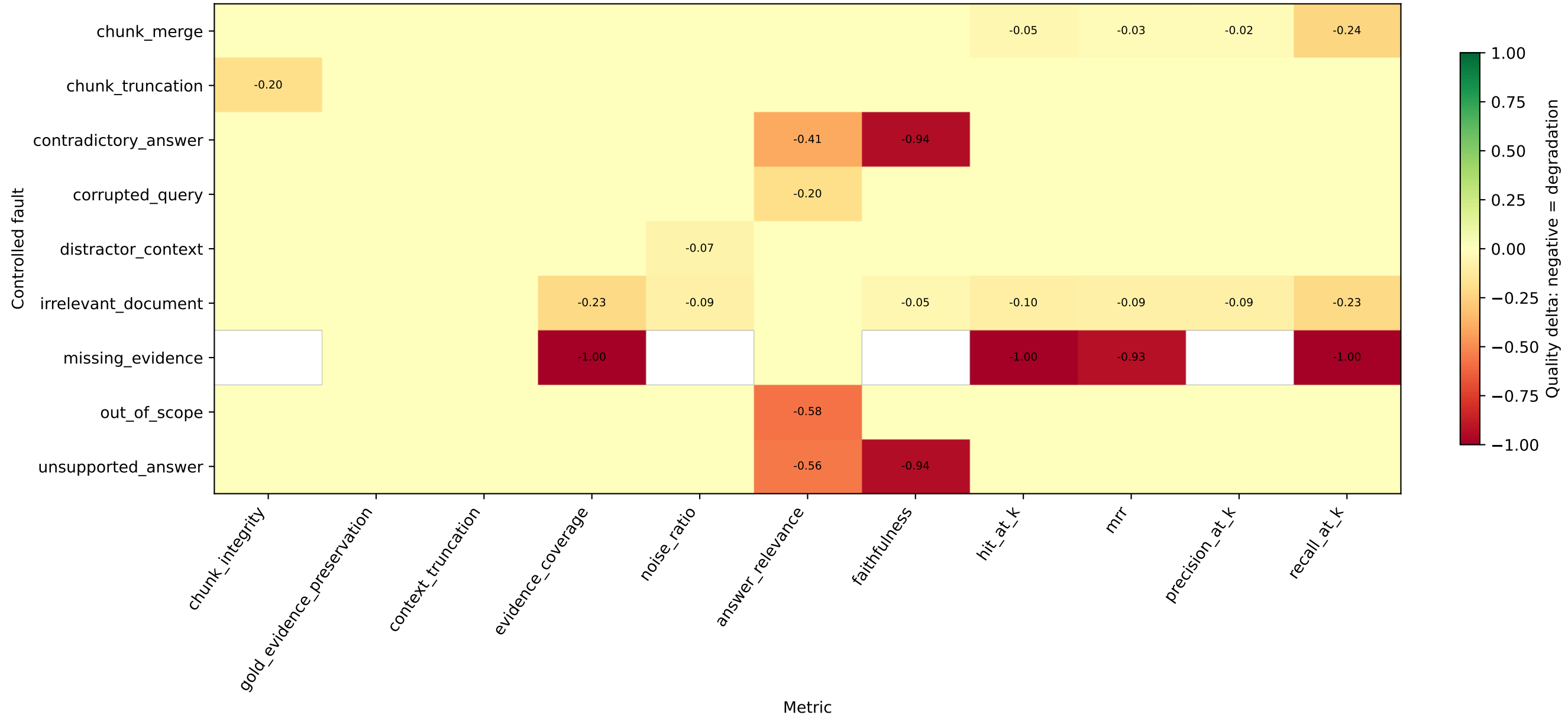
Controlled-failure metric sensitivity Quality-normalized paired delta (fault - healthy) BM25
