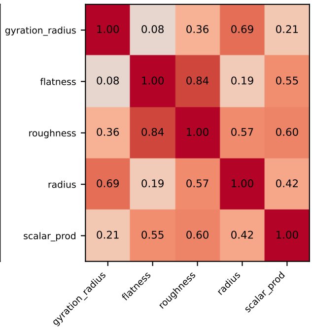
Spearman
