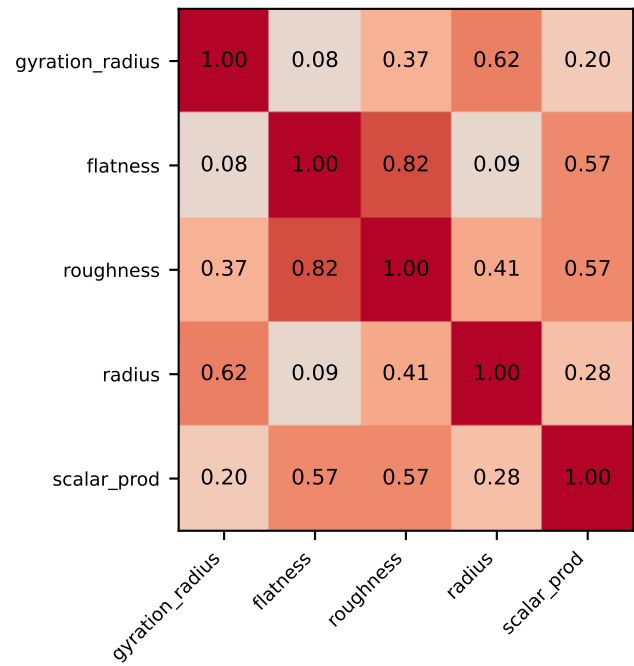
Pearson
