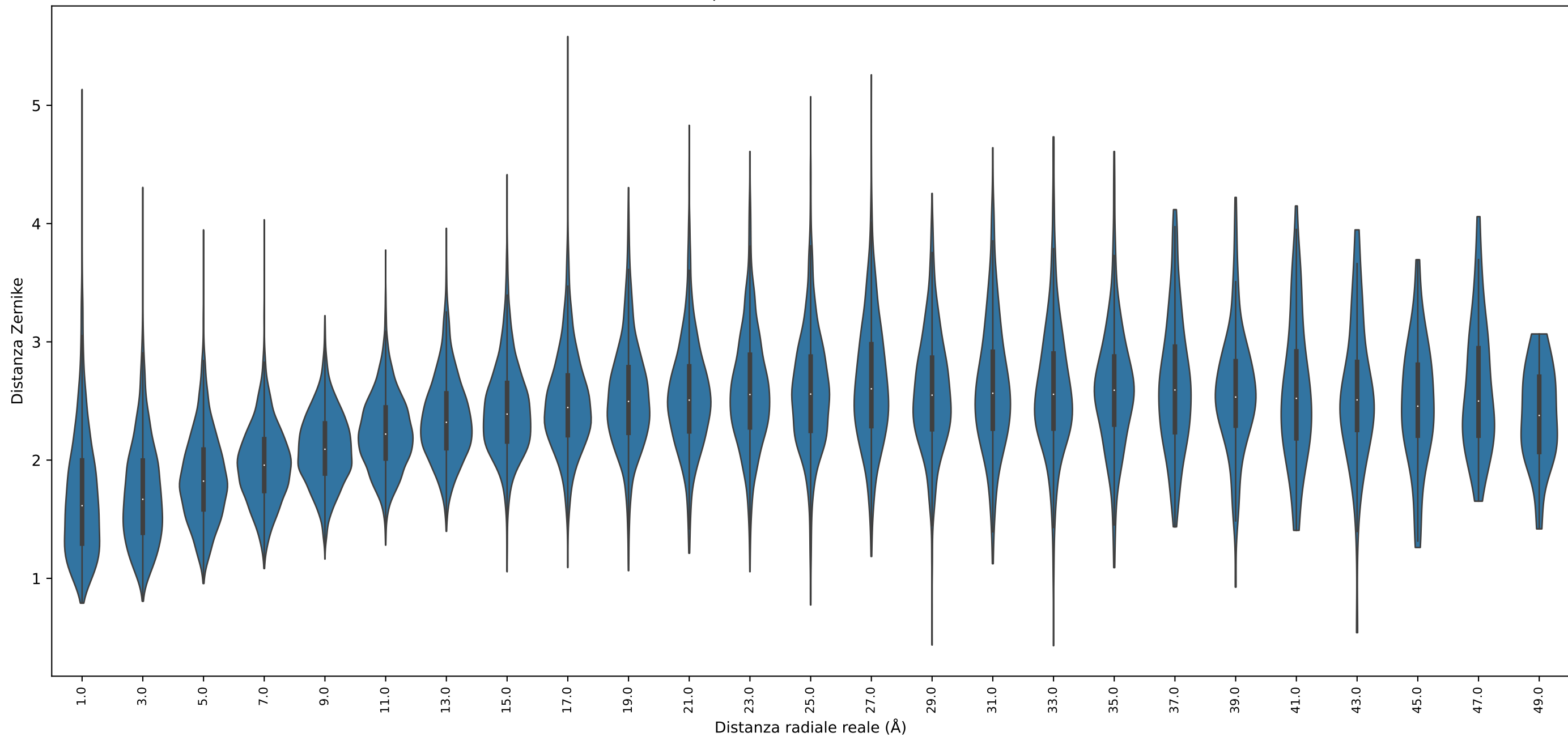
Violin plot distanza Zernike native
