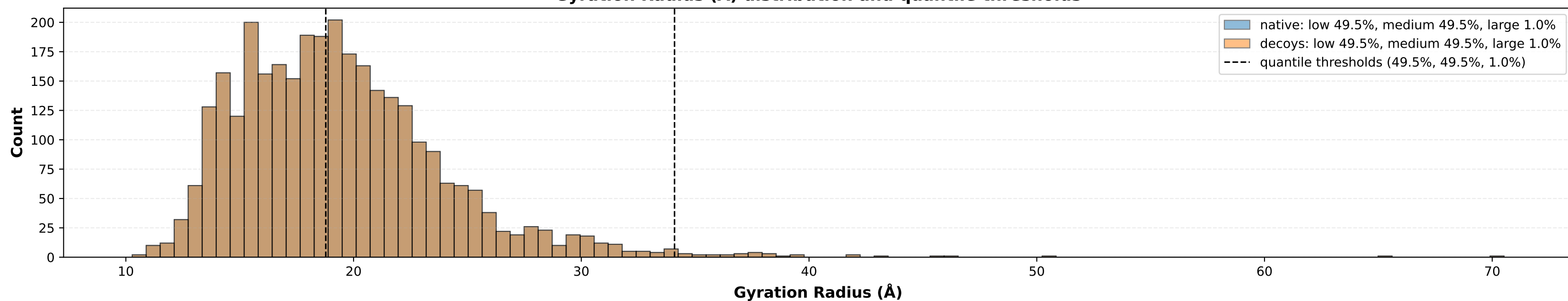
Gyration Radius (Å) - Low quantile - Physical Distance per Ring
