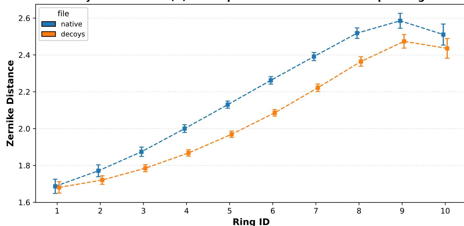
Gyration Radius (Å) - Medium quantile - Zernike Distance per Ring
