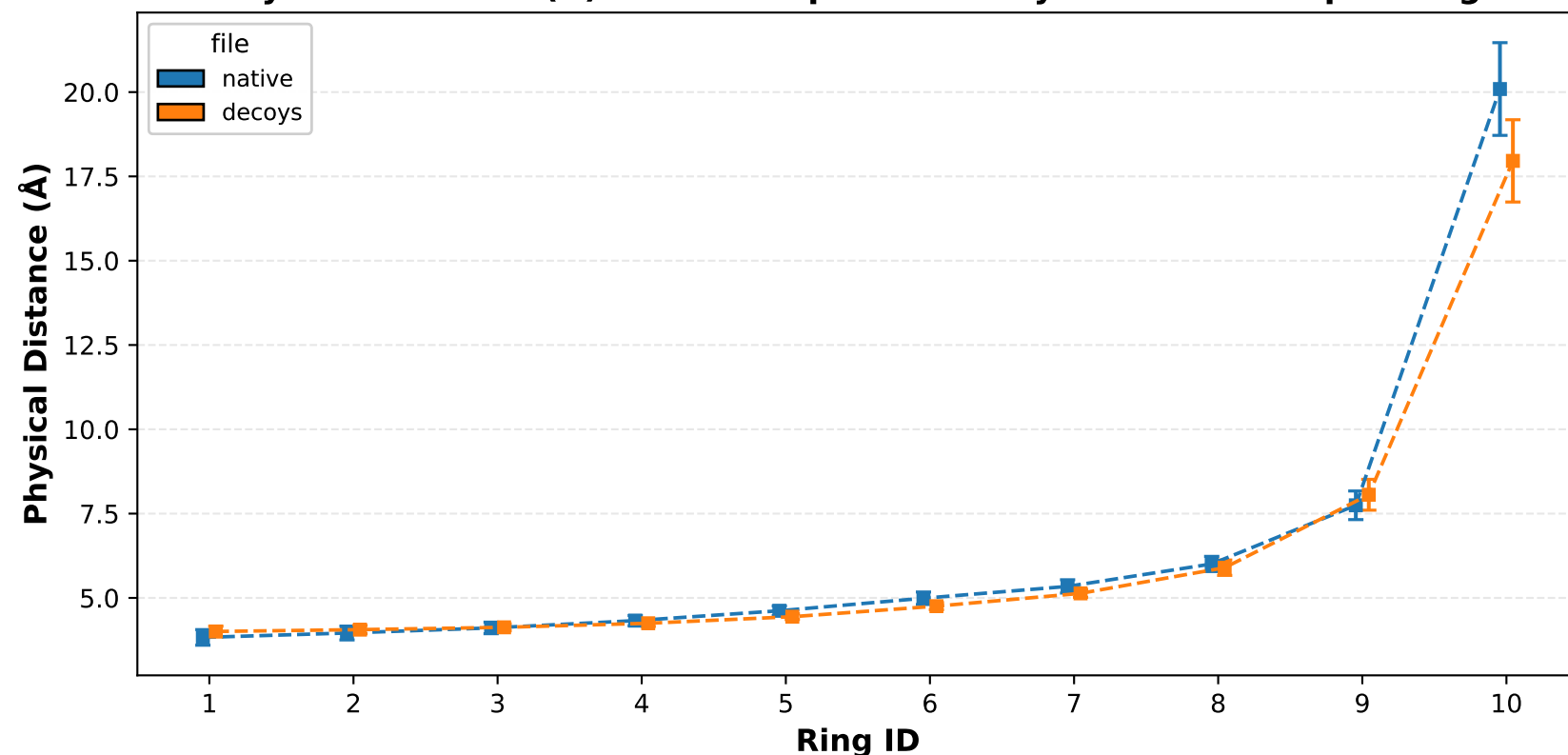
Gyration Radius (Å) - Large quantile - Physical Distance per Ring
