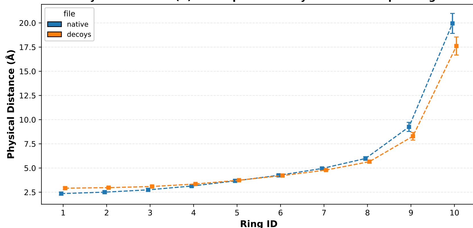
Gyration Radius (Å) - Medium quantile - Physical Distance per Ring
