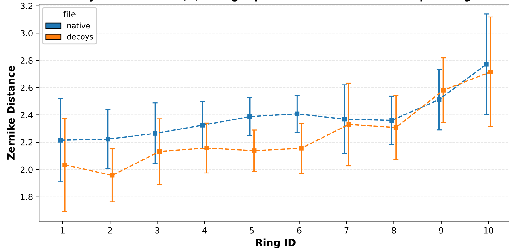
Gyration Radius (Å) - Large quantile - Zernike Distance per Ring
