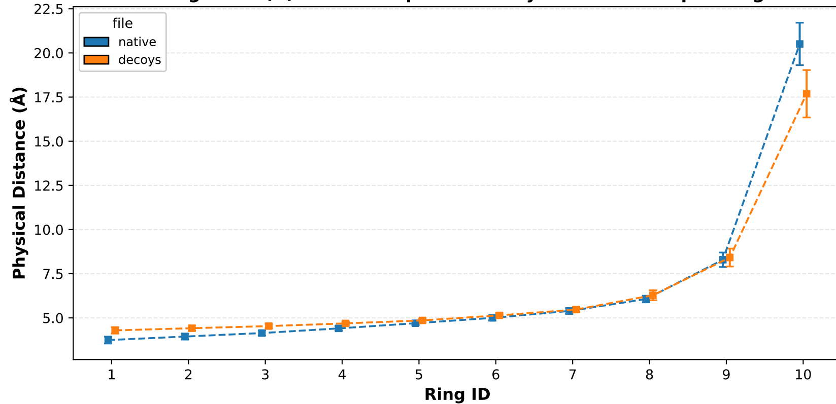
Roughness (Å) - Large quantile - Physical Distance per Ring
