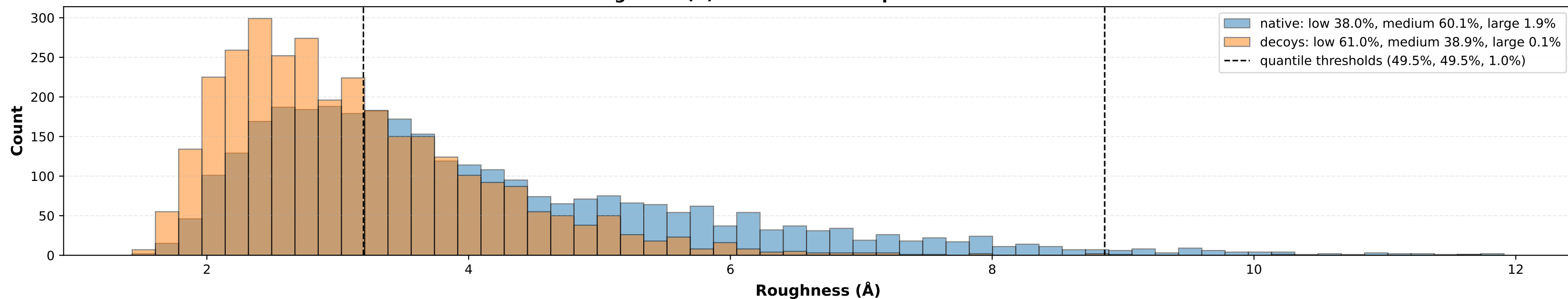
Roughness (Å) - Low quantile - Physical Distance per Ring
