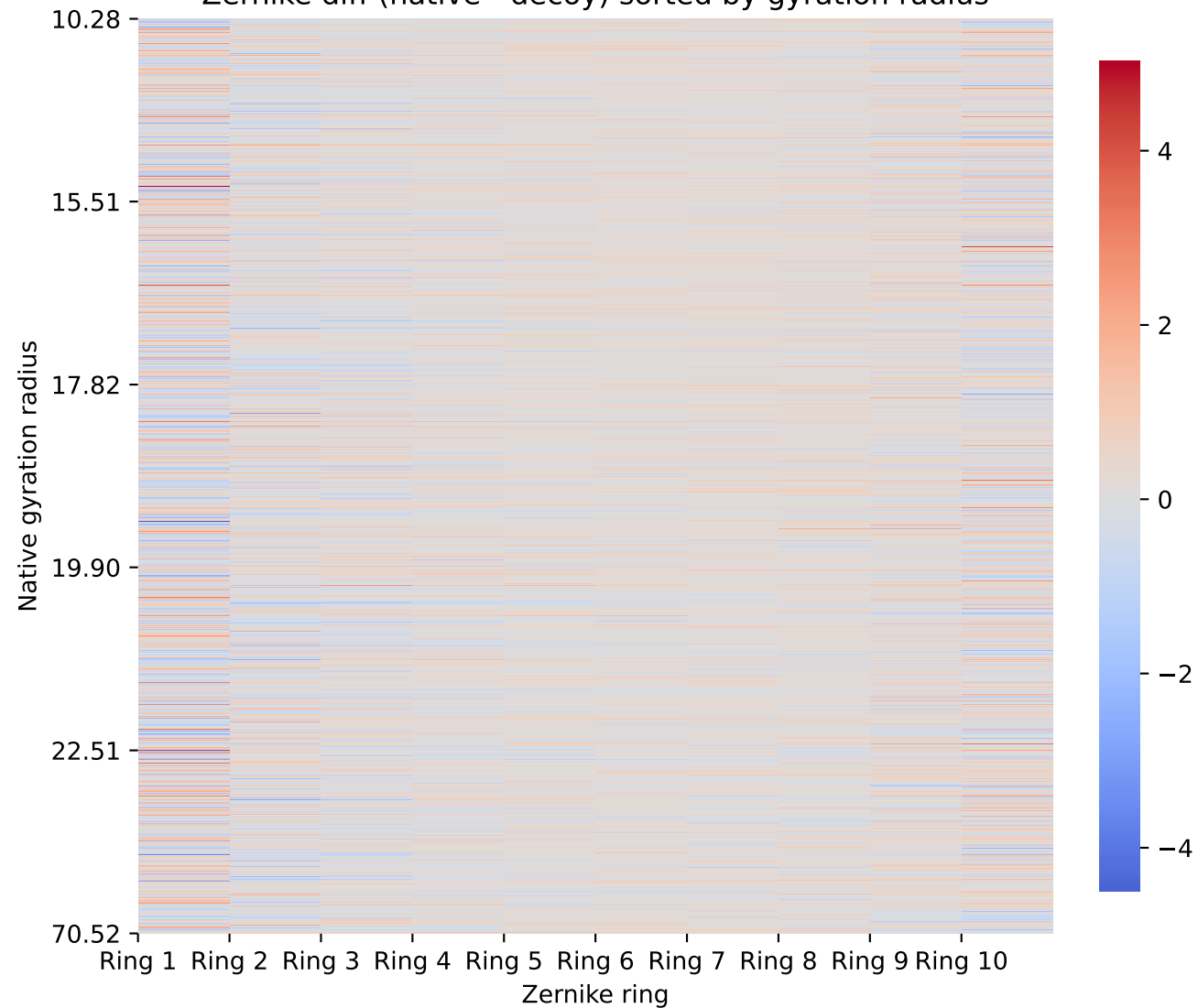
Zernike diff (native - decoy) sorted by gyration radius
