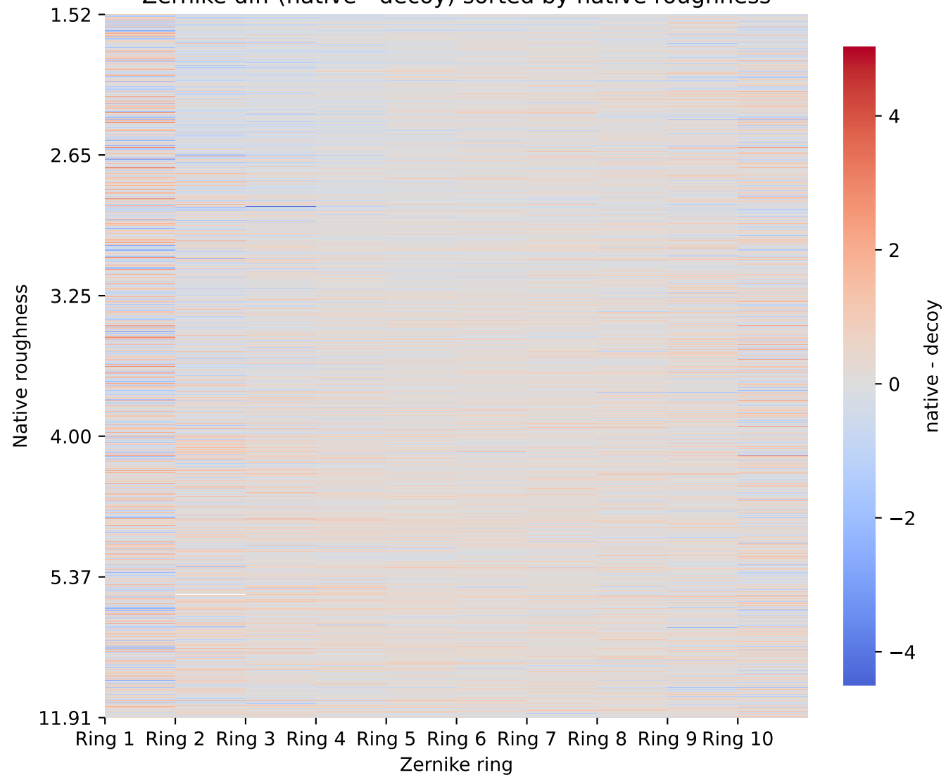
Zernike diff (native - decoy) sorted by native roughness
