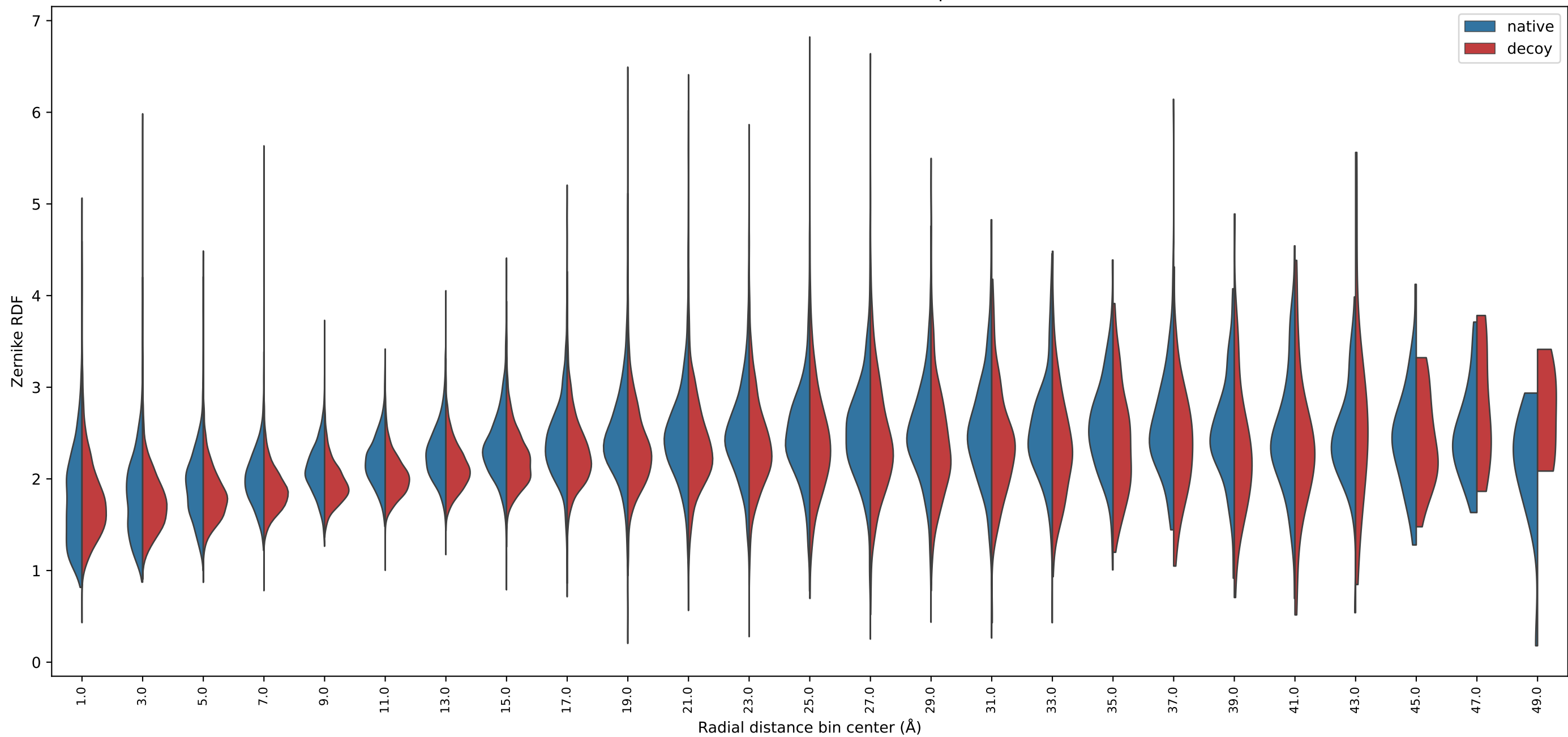
Zernike RDF - actual radial distance (split violin)
