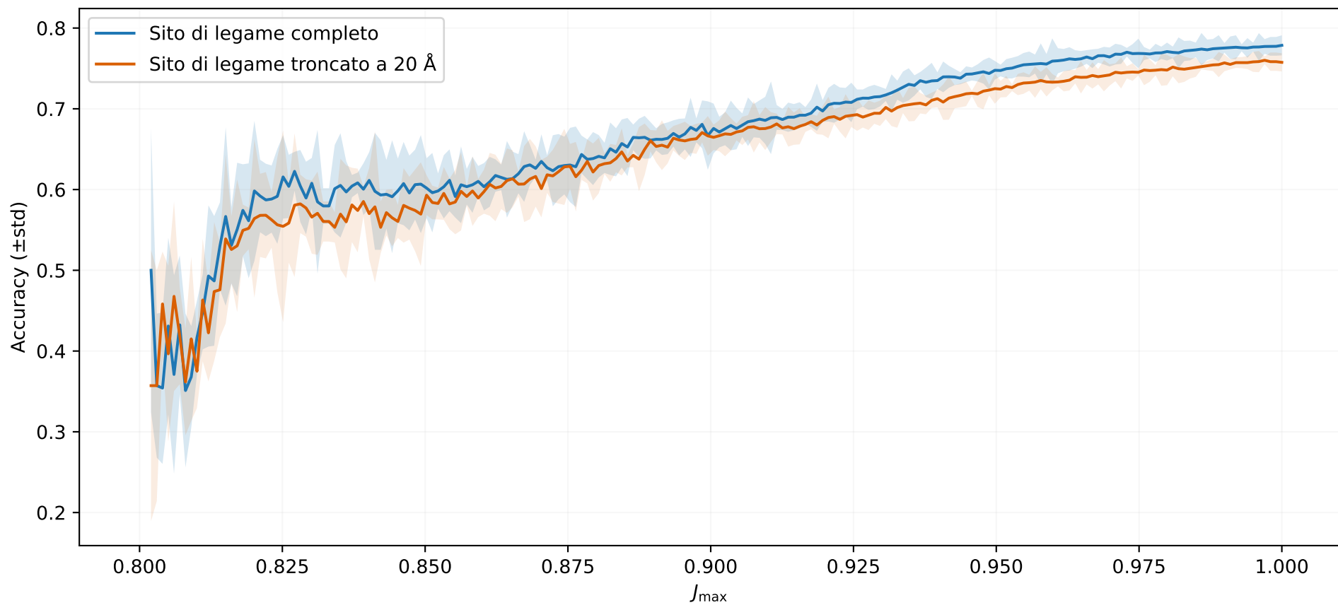
Accuracy vs J_{\max}
