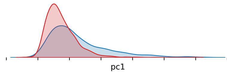
Roughness RDF
