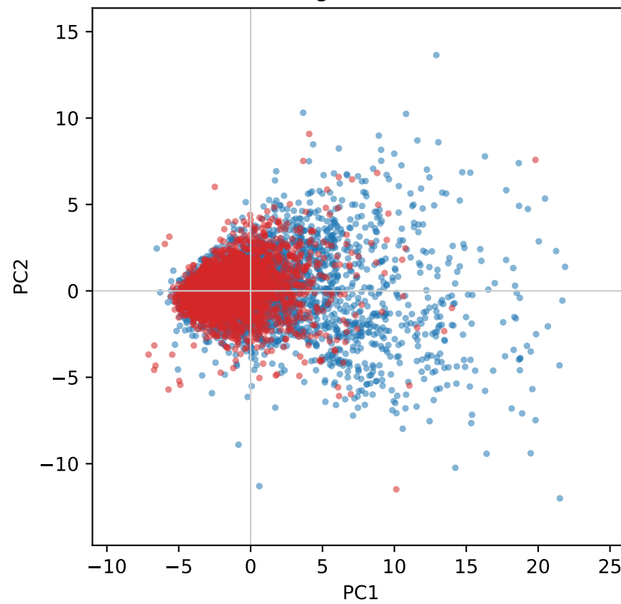
Roughness RDF
