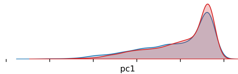
Physical RDF
