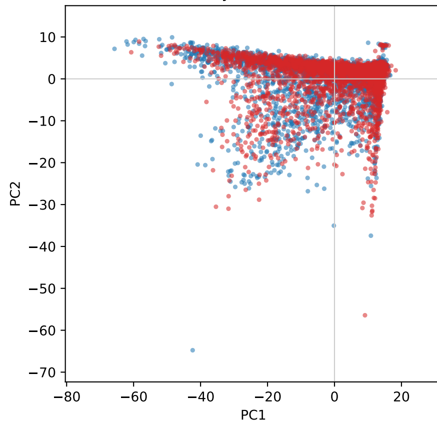
Physical RDF
