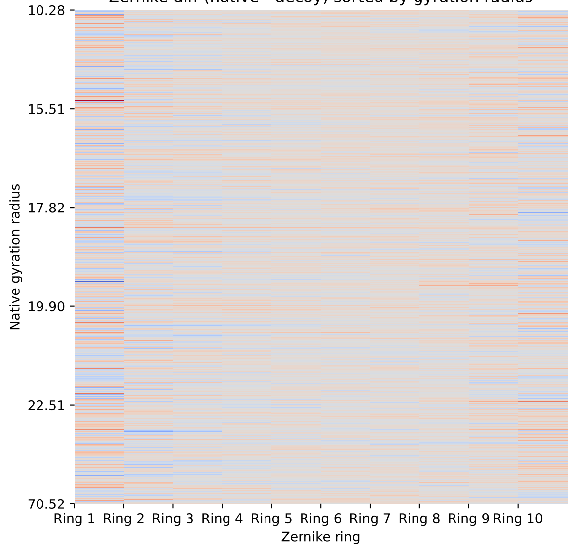
Zernike diff (native - decoy) sorted by gyration radius
