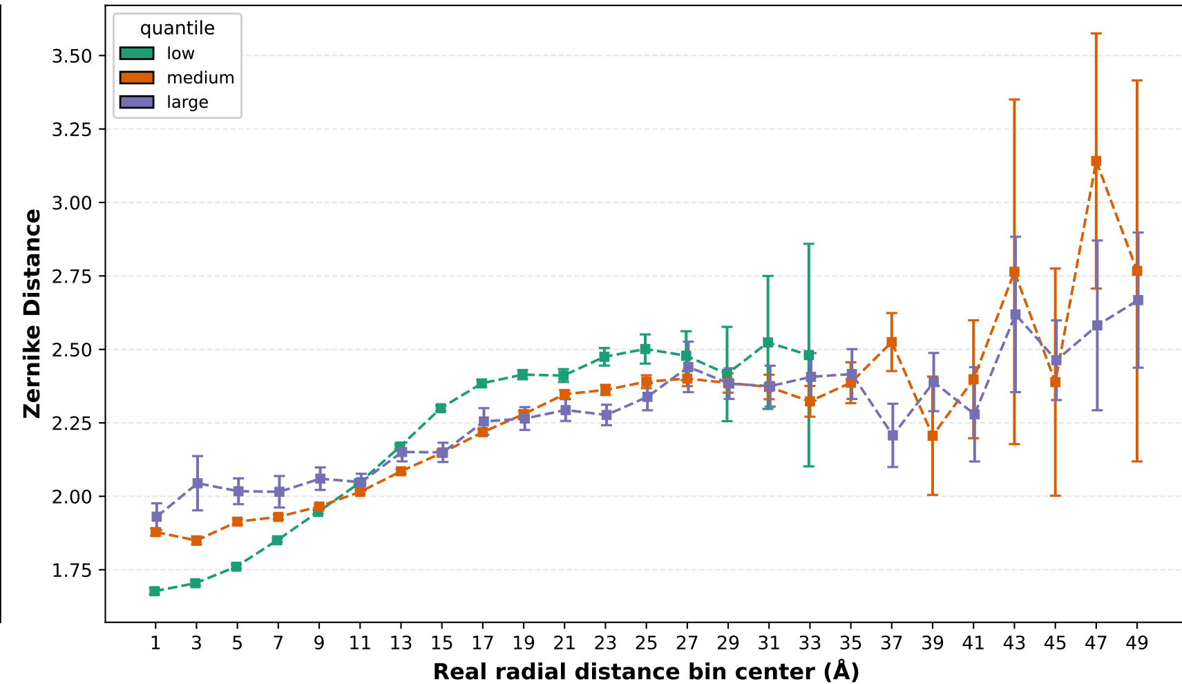
gyration_radius - Zernike Distance per Ring
