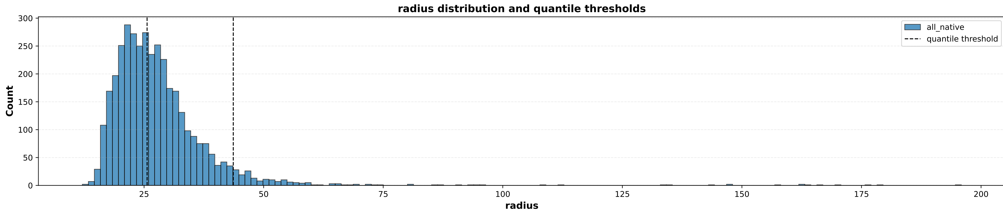
radius quantiles with RDFs (all_native)
