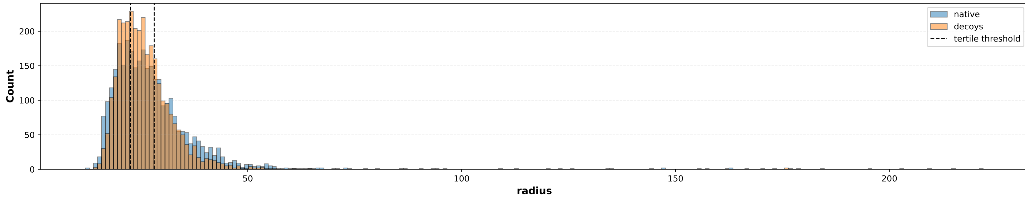
radius distribution and tertile thresholds
