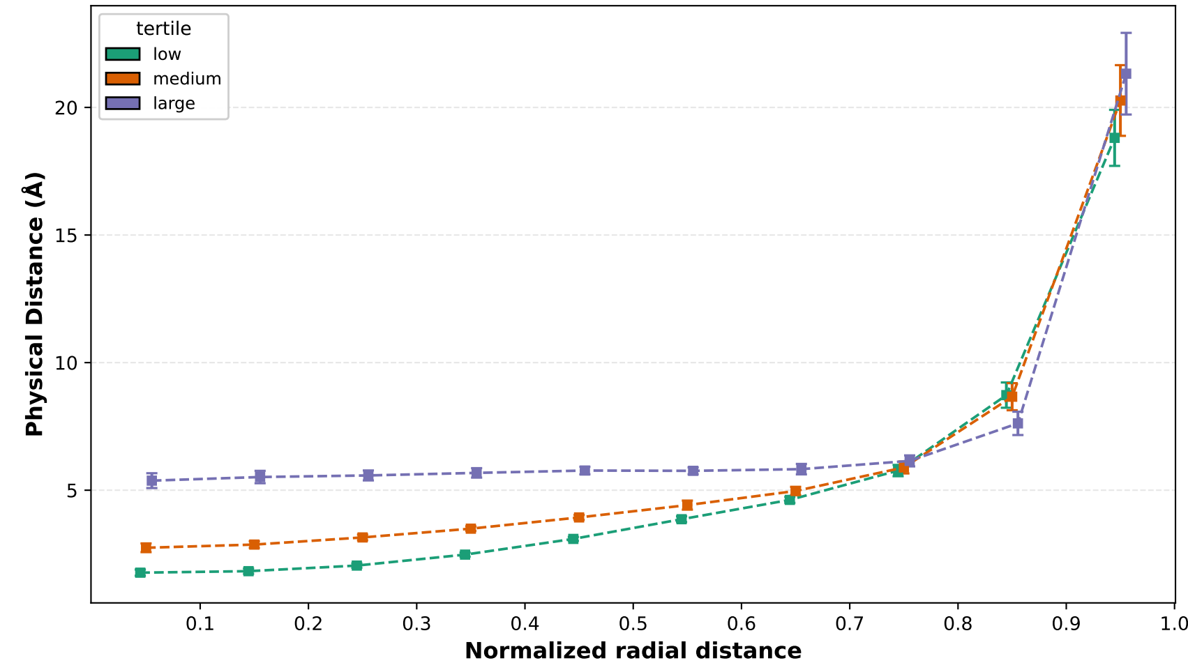
Physical distance RDF
