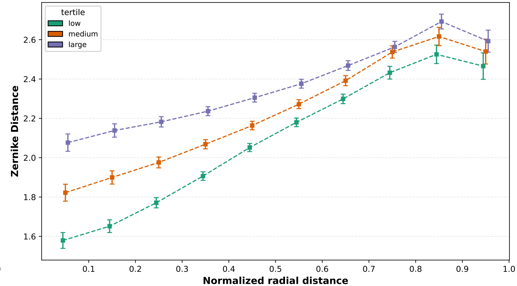
Zernike distance RDF
